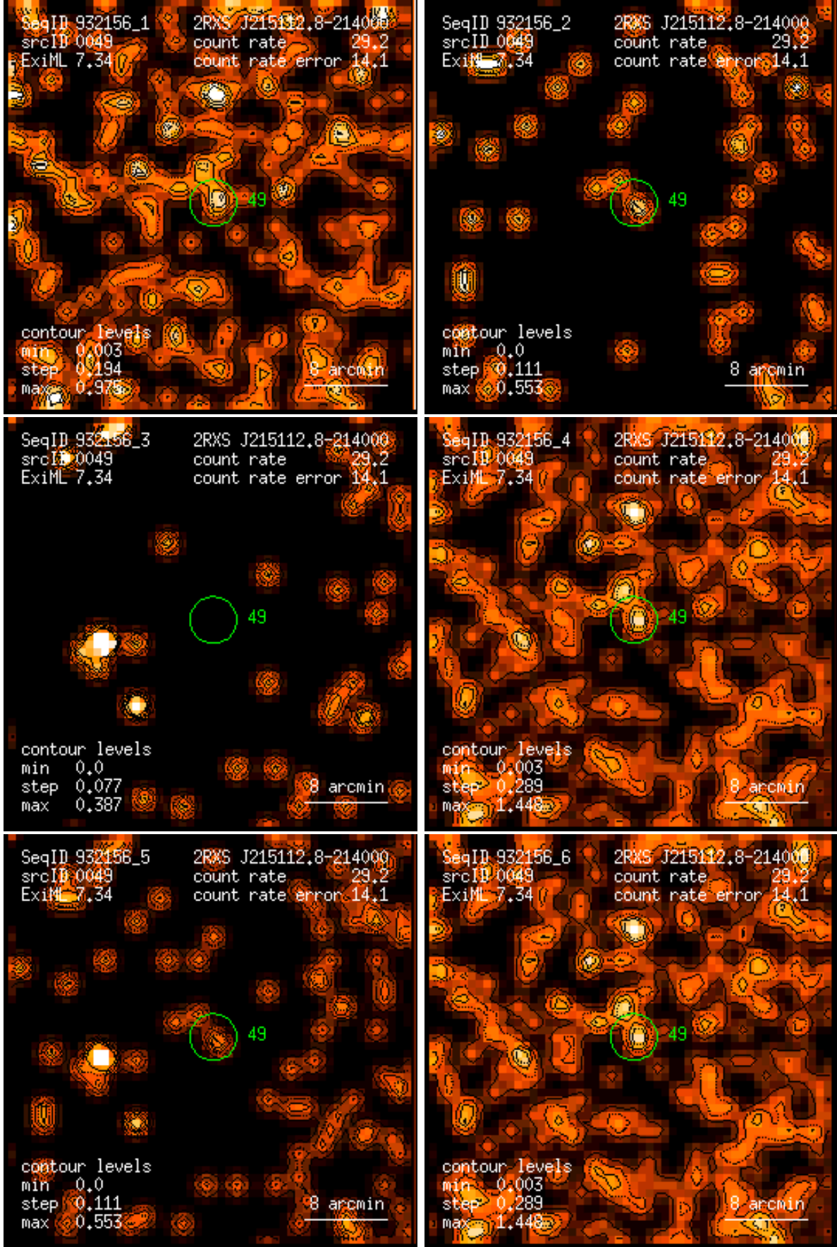
Figure 49: RASS 932156: detection 0049: band rate images, Gaussian filter: (1) PSPC channels 11 – 41, (2) 52 – 90, (3) 91 – 201, (4) 11 – 235, (5) 52 – 201, (6) 11 – 201. Broad band rates in counts/ks. Band rate contour levels in counts/ks/arcmin 2 .
