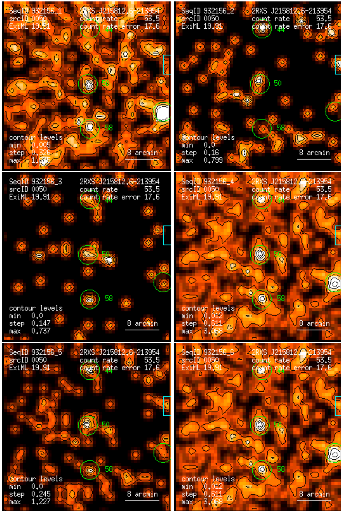
Figure 50: RASS 932156: detection 0050: band rate images, Gaussian filter: (1) PSPC channels 11 – 41, (2) 52 – 90, (3) 91 – 201, (4) 11 – 235, (5) 52 – 201, (6) 11 – 201. Broad band rates in counts/ks. Band rate contour levels in counts/ks/arcmin 2 .
