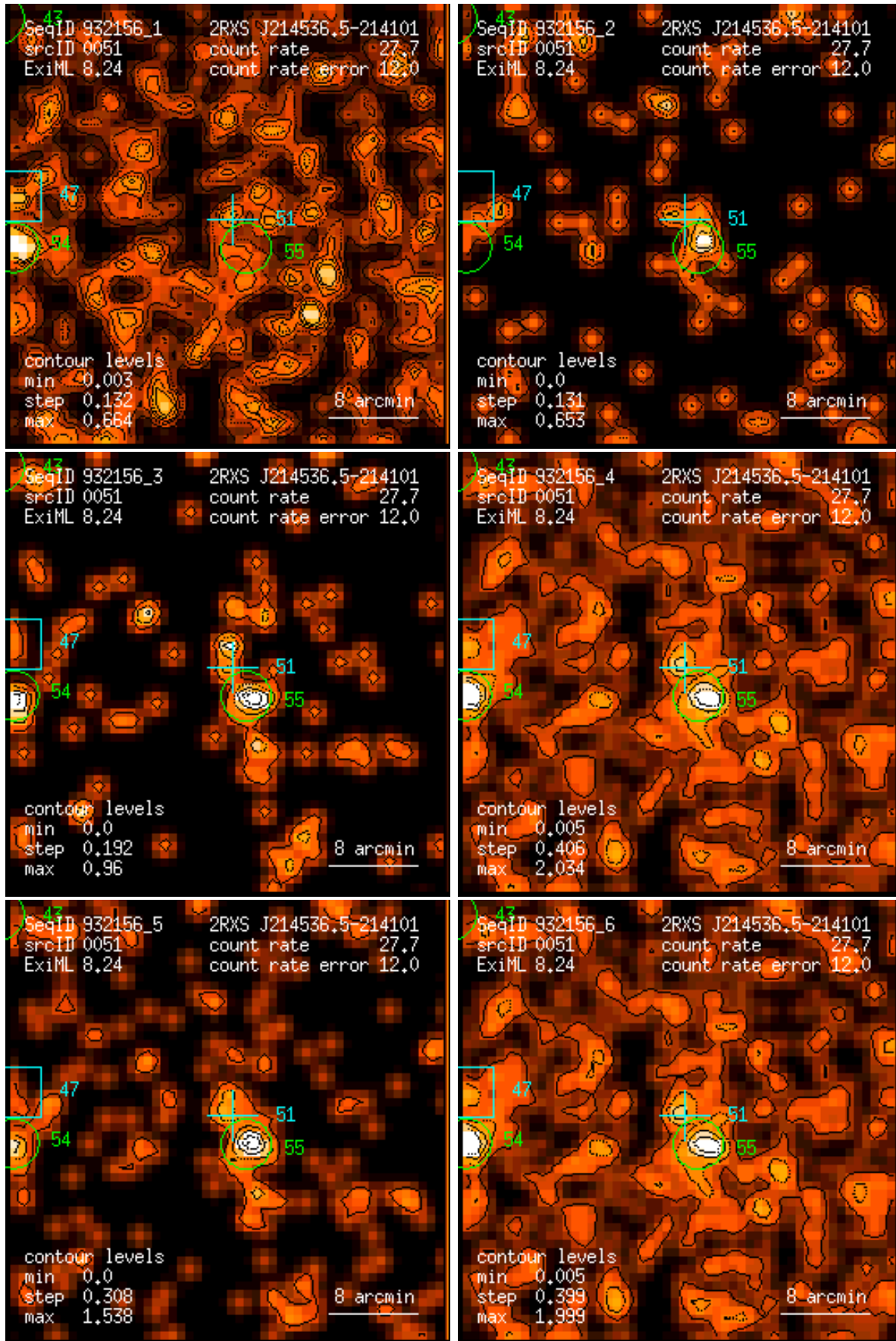
Figure 51: RASS 932156: detection 0051: band rate images, Gaussian filter: (1) PSPC channels 11 – 41, (2) 52 – 90, (3) 91 – 201, (4) 11 – 235, (5) 52 – 201, (6) 11 – 201. Broad band rates in counts/ks. Band rate contour levels in counts/ks/arcmin 2 .
