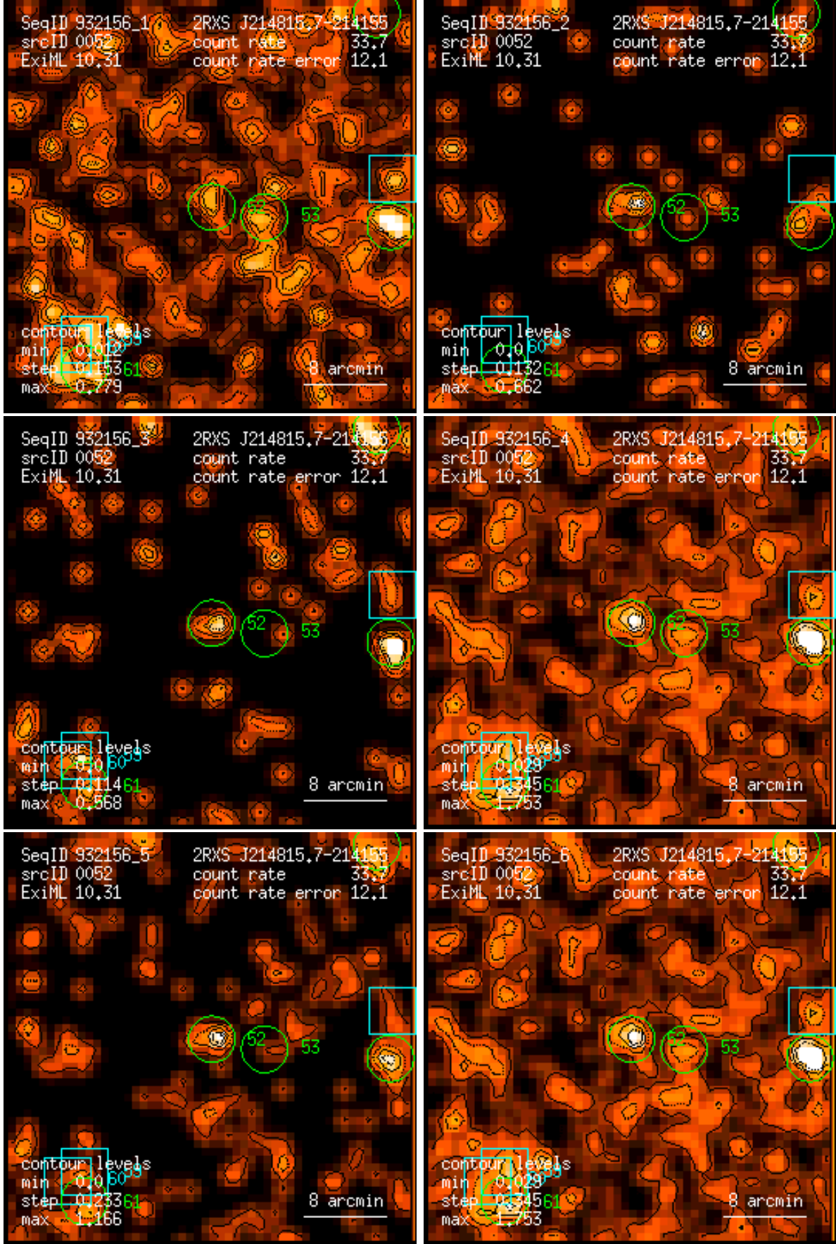
Figure 52: RASS 932156: detection 0052: band rate images, Gaussian filter: (1) PSPC channels 11 – 41, (2) 52 – 90, (3) 91 – 201, (4) 11 – 235, (5) 52 – 201, (6) 11 – 201. Broad band rates in counts/ks. Band rate contour levels in counts/ks/arcmin 2 .
