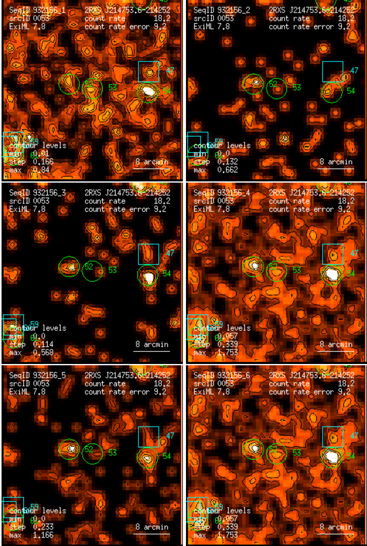
Figure 53: RASS 932156: detection 0053: band rate images, Gaussian filter: (1) PSPC channels 11 – 41, (2) 52 – 90, (3) 91 – 201, (4) 11 – 235, (5) 52 – 201, (6) 11 – 201. Broad band rates in counts/ks. Band rate contour levels in counts/ks/arcmin 2 .
