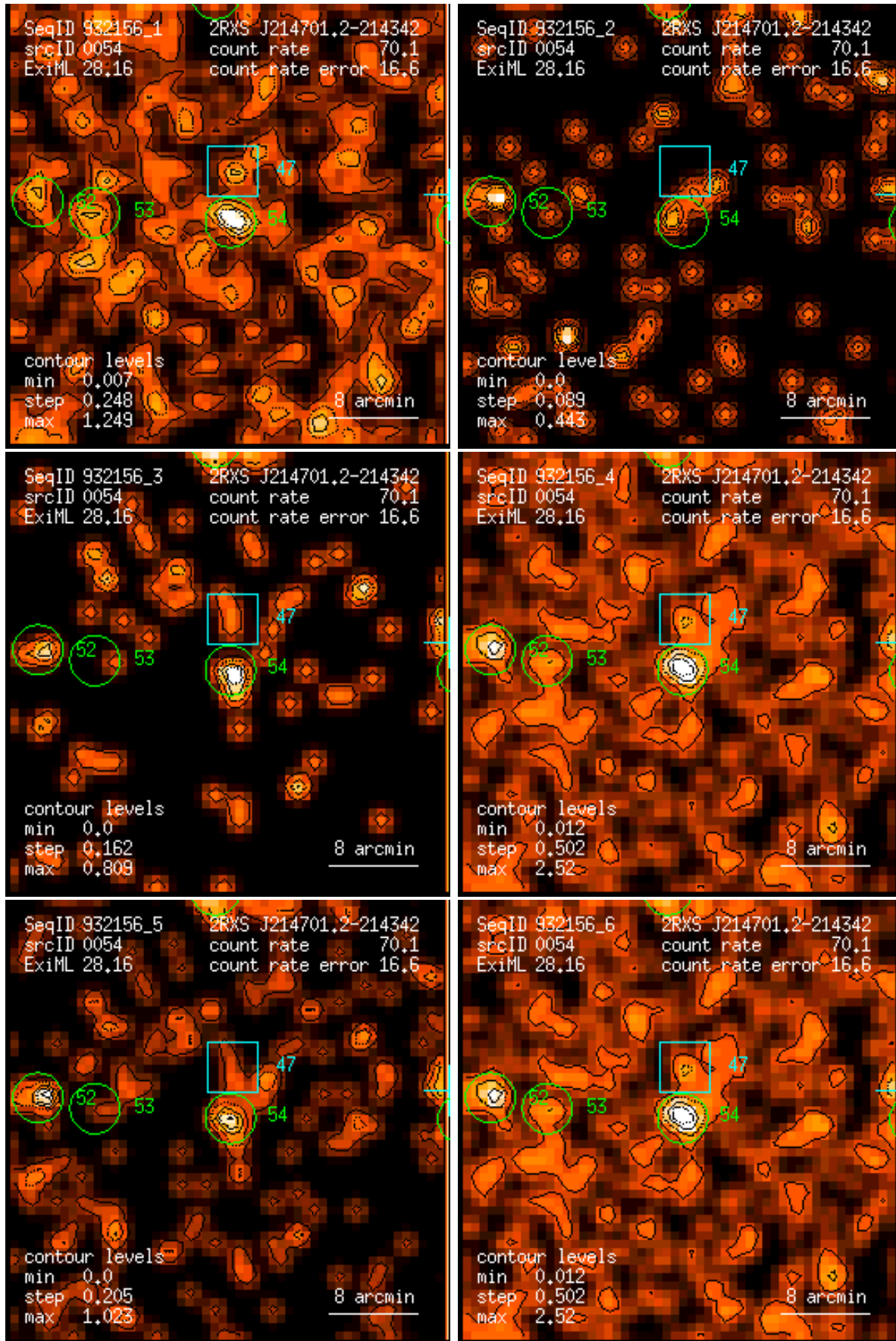
Figure 54: RASS 932156: detection 0054: band rate images, Gaussian filter: (1) PSPC channels 11 – 41, (2) 52 – 90, (3) 91 – 201, (4) 11 – 235, (5) 52 – 201, (6) 11 – 201. Broad band rates in counts/ks. Band rate contour levels in counts/ks/arcmin 2 .
