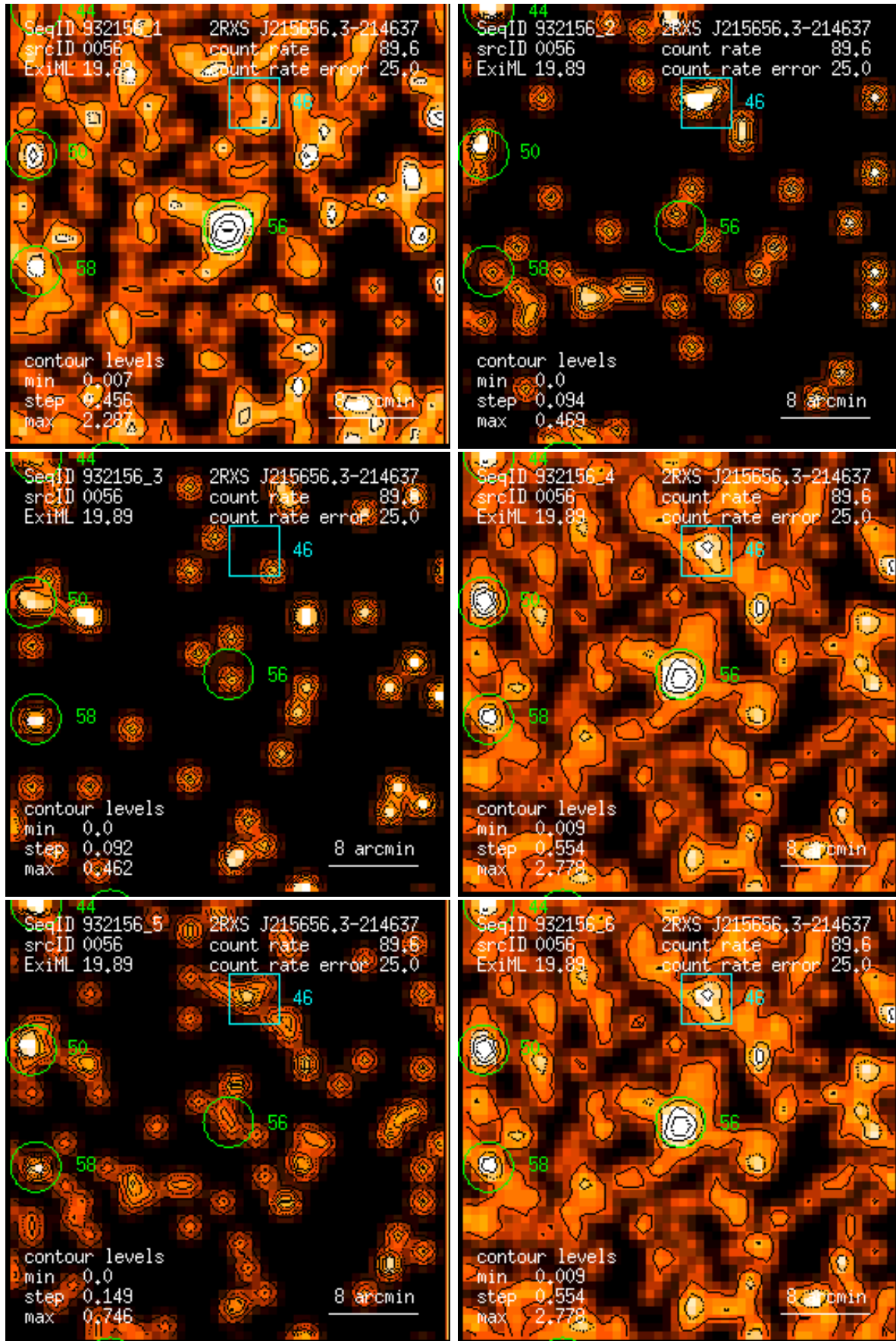
Figure 56: RASS 932156: detection 0056: band rate images, Gaussian filter: (1) PSPC channels 11 – 41, (2) 52 – 90, (3) 91 – 201, (4) 11 – 235, (5) 52 – 201, (6) 11 – 201. Broad band rates in counts/ks. Band rate contour levels in counts/ks/arcmin 2 .
