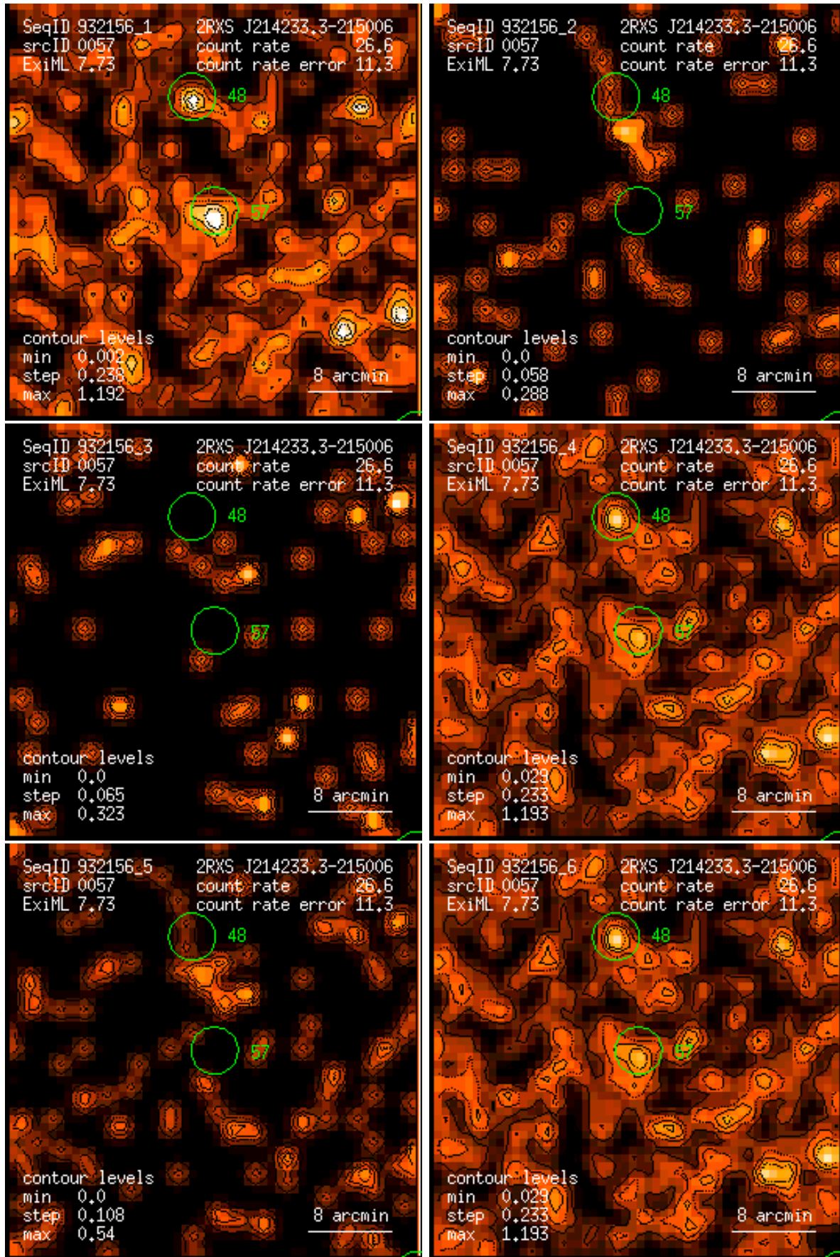
Figure 57: RASS 932156: detection 0057: band rate images, Gaussian filter: (1) PSPC channels 11 – 41, (2) 52 – 90, (3) 91 – 201, (4) 11 – 235, (5) 52 – 201, (6) 11 – 201. Broad band rates in counts/ks. Band rate contour levels in counts/ks/arcmin 2 .
