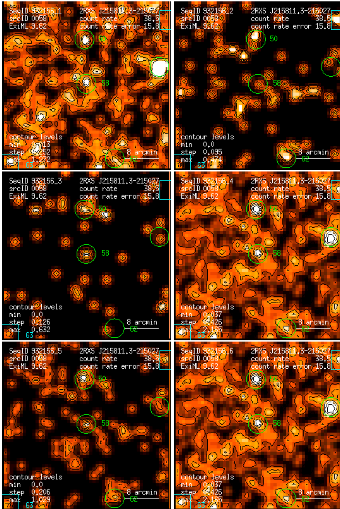
Figure 58: RASS 932156: detection 0058: band rate images, Gaussian filter: (1) PSPC channels 11 – 41, (2) 52 – 90, (3) 91 – 201, (4) 11 – 235, (5) 52 – 201, (6) 11 – 201. Broad band rates in counts/ks. Band rate contour levels in counts/ks/arcmin 2 .
