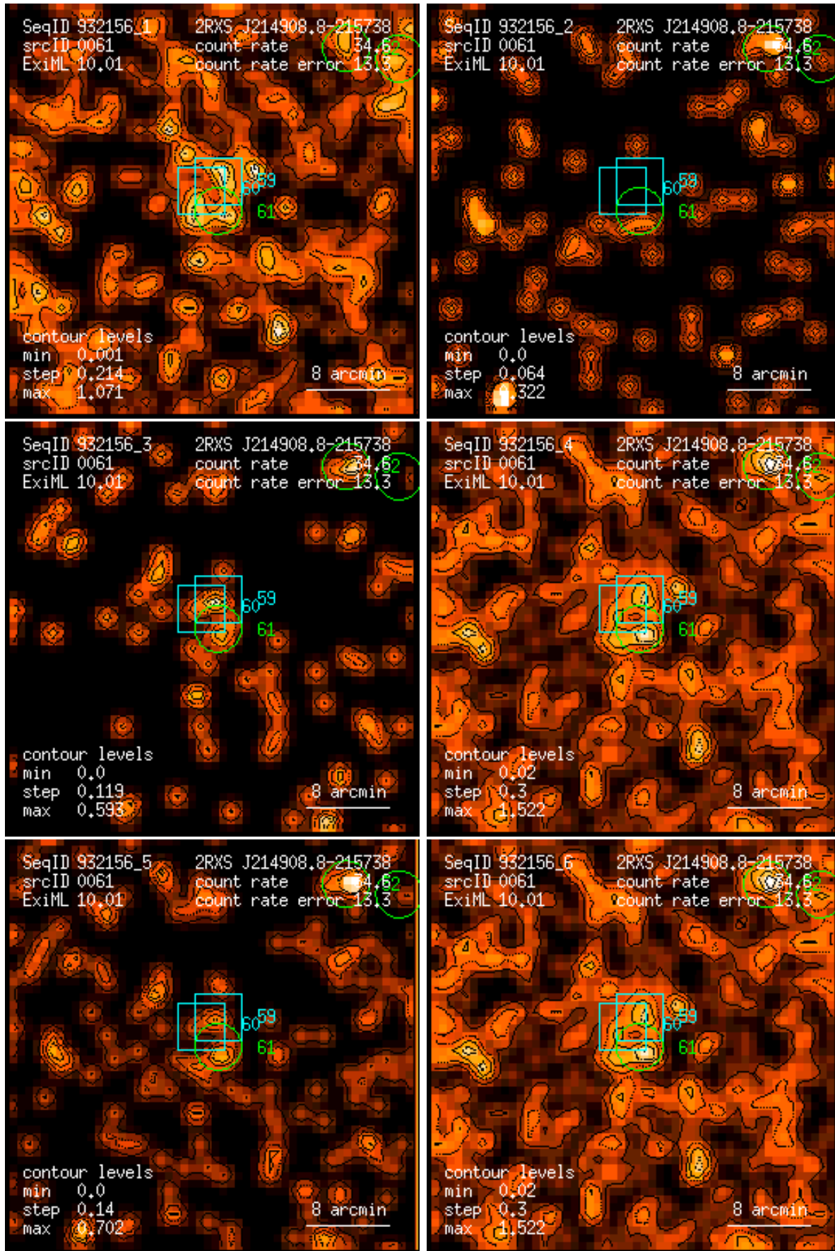
Figure 61: RASS 932156: detection 0061: band rate images, Gaussian filter: (1) PSPC channels 11 – 41, (2) 52 – 90, (3) 91 – 201, (4) 11 – 235, (5) 52 – 201, (6) 11 – 201. Broad band rates in counts/ks. Band rate contour levels in counts/ks/arcmin 2 .
