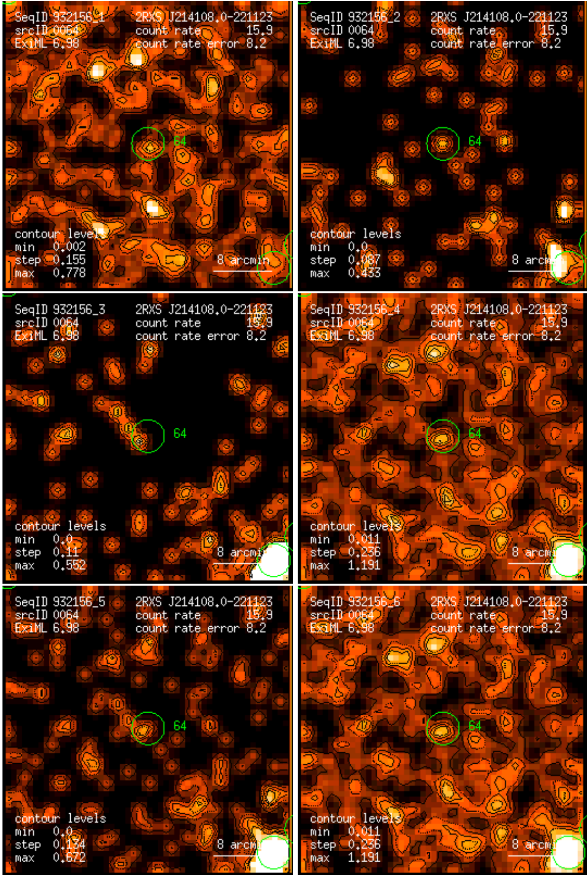
Figure 64: RASS 932156: detection 0064: band rate images, Gaussian filter: (1) PSPC channels 11 – 41, (2) 52 – 90, (3) 91 – 201, (4) 11 – 235, (5) 52 – 201, (6) 11 – 201. Broad band rates in counts/ks. Band rate contour levels in counts/ks/arcmin 2 .
