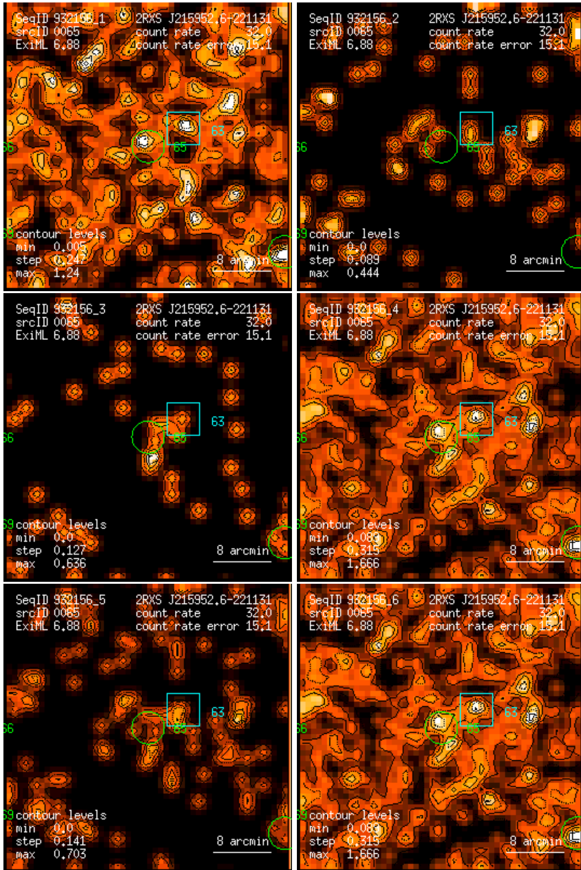
Figure 65: RASS 932156: detection 0065: band rate images, Gaussian filter: (1) PSPC channels 11 – 41, (2) 52 – 90, (3) 91 – 201, (4) 11 – 235, (5) 52 – 201, (6) 11 – 201. Broad band rates in counts/ks. Band rate contour levels in counts/ks/arcmin 2 .
