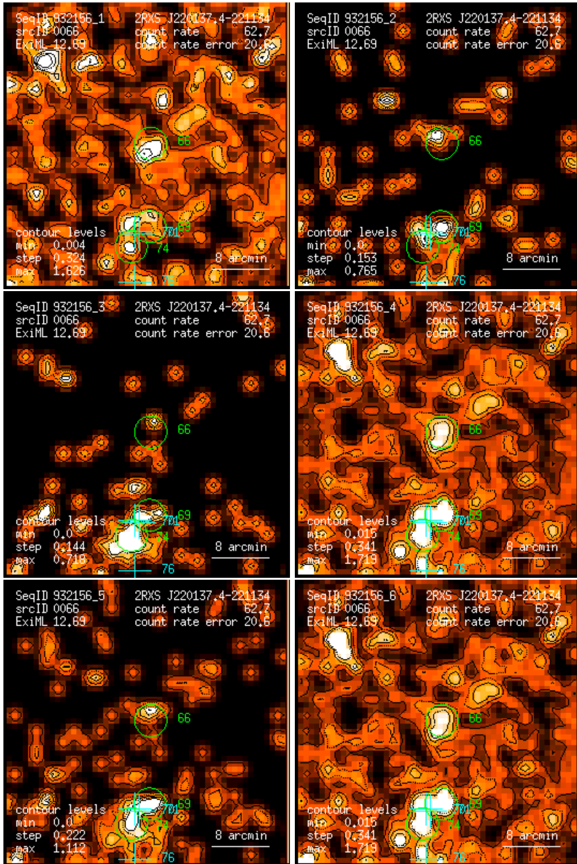
Figure 66: RASS 932156: detection 0066: band rate images, Gaussian filter: (1) PSPC channels 11 – 41, (2) 52 – 90, (3) 91 – 201, (4) 11 – 235, (5) 52 – 201, (6) 11 – 201. Broad band rates in counts/ks. Band rate contour levels in counts/ks/arcmin 2 .
