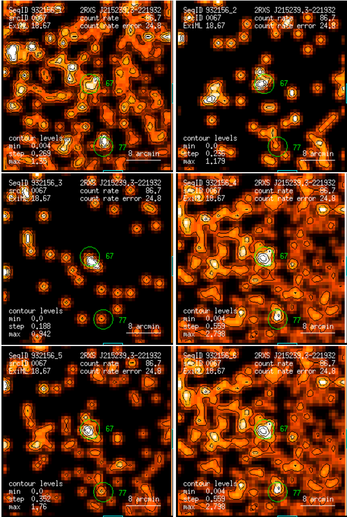
Figure 67: RASS 932156: detection 0067: band rate images, Gaussian filter: (1) PSPC channels 11 – 41, (2) 52 – 90, (3) 91 – 201, (4) 11 – 235, (5) 52 – 201, (6) 11 – 201. Broad band rates in counts/ks. Band rate contour levels in counts/ks/arcmin 2 .
