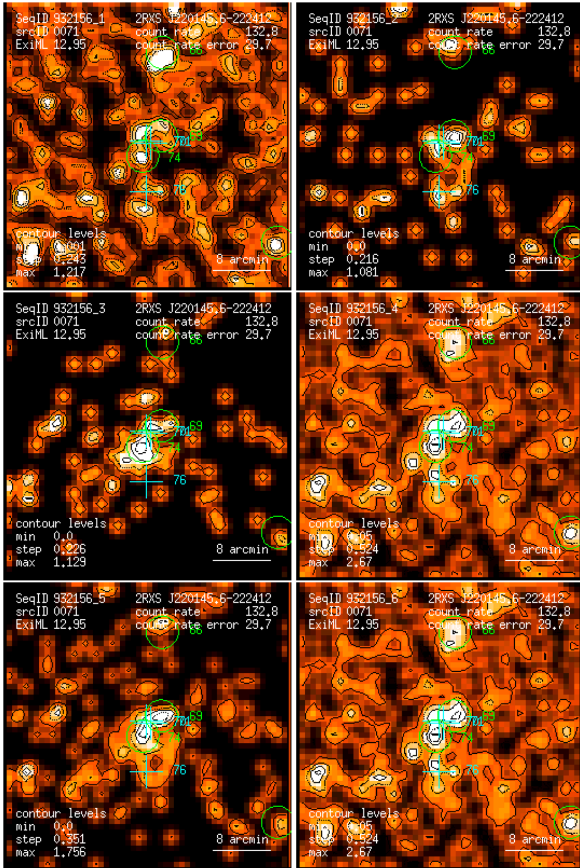
Figure 71: RASS 932156: detection 0071: band rate images, Gaussian filter: (1) PSPC channels 11 – 41, (2) 52 – 90, (3) 91 – 201, (4) 11 – 235, (5) 52 – 201, (6) 11 – 201. Broad band rates in counts/ks. Band rate contour levels in counts/ks/arcmin 2 .
