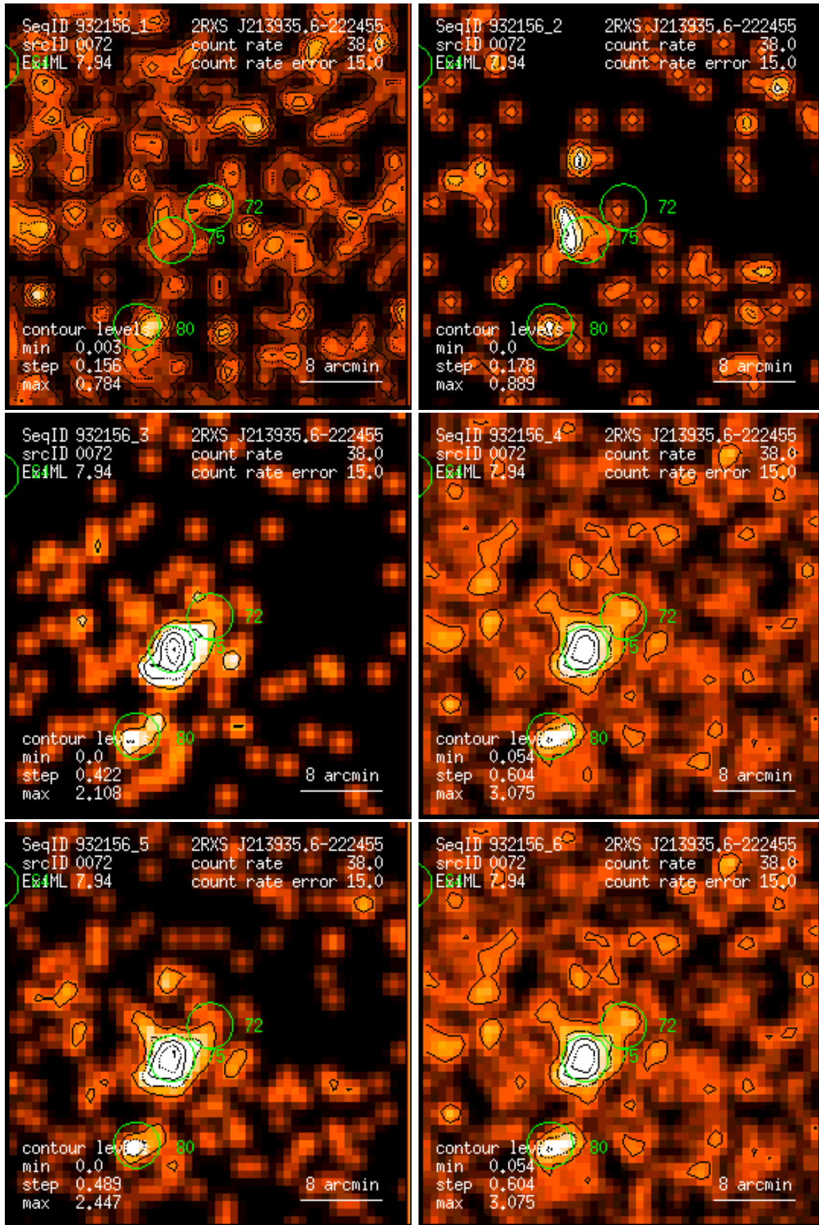
Figure 72: RASS 932156: detection 0072: band rate images, Gaussian filter: (1) PSPC channels 11 – 41, (2) 52 – 90, (3) 91 – 201, (4) 11 – 235, (5) 52 – 201, (6) 11 – 201. Broad band rates in counts/ks. Band rate contour levels in counts/ks/arcmin 2 .
