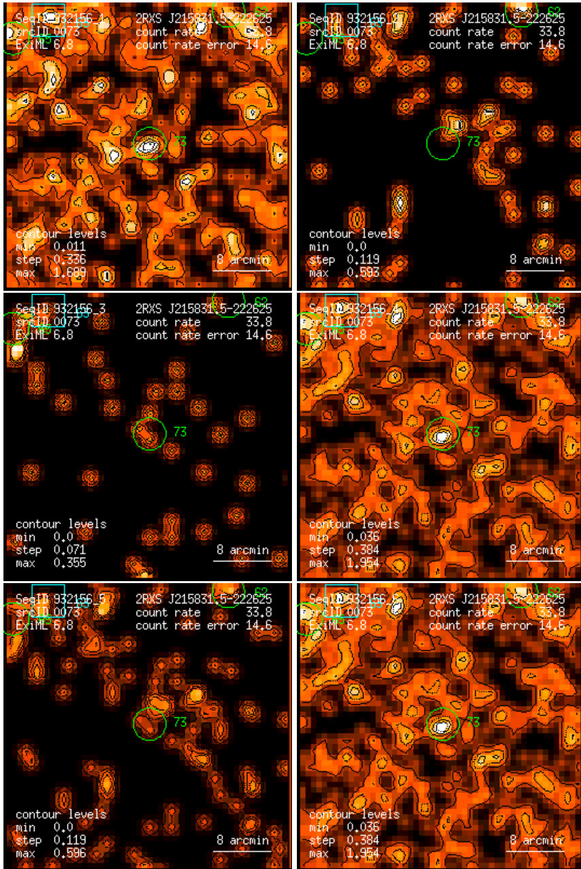
Figure 73: RASS 932156: detection 0073: band rate images, Gaussian filter: (1) PSPC channels 11 – 41, (2) 52 – 90, (3) 91 – 201, (4) 11 – 235, (5) 52 – 201, (6) 11 – 201. Broad band rates in counts/ks. Band rate contour levels in counts/ks/arcmin 2 .
