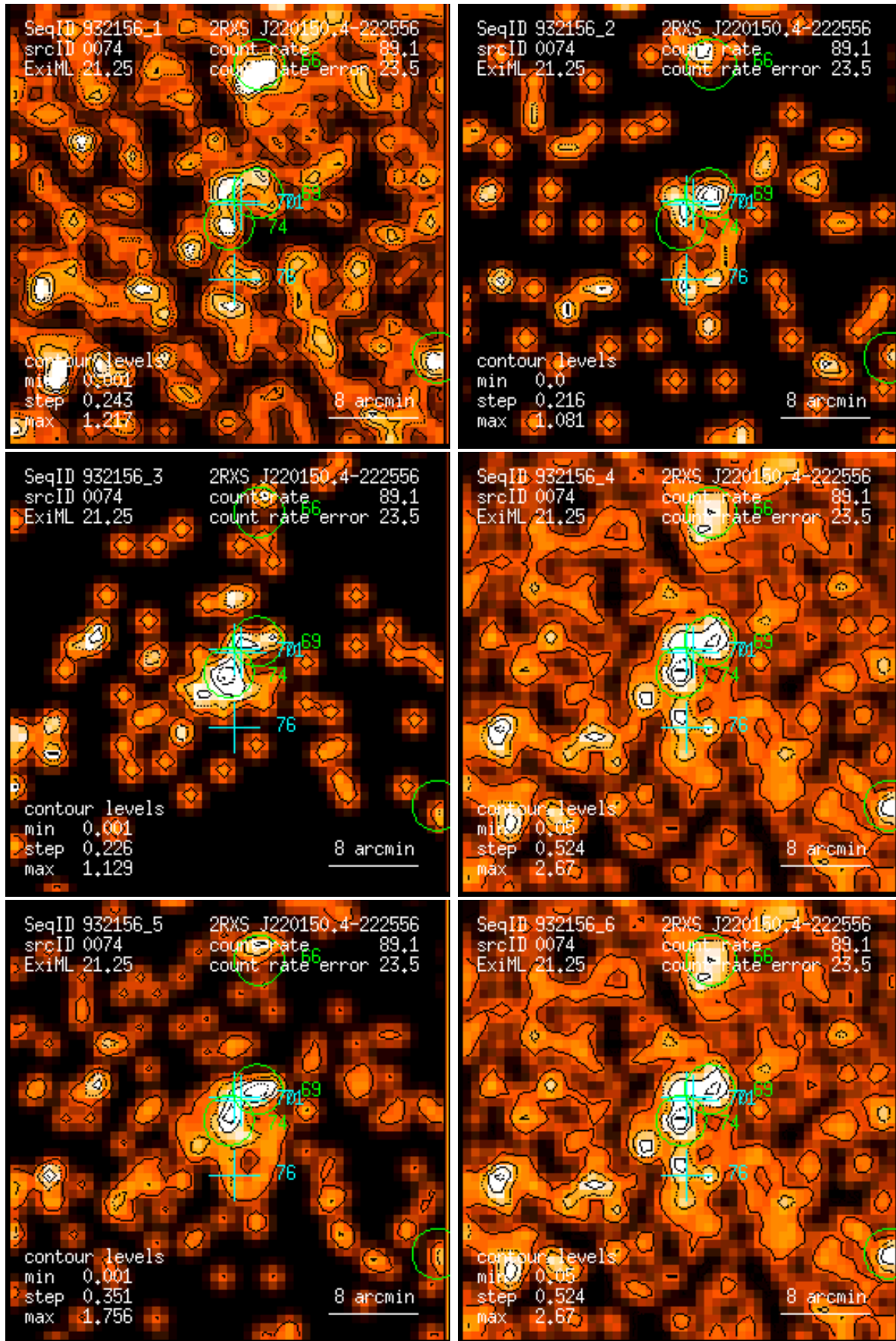
Figure 74: RASS 932156: detection 0074: band rate images, Gaussian filter: (1) PSPC channels 11 – 41, (2) 52 – 90, (3) 91 – 201, (4) 11 – 235, (5) 52 – 201, (6) 11 – 201. Broad band rates in counts/ks. Band rate contour levels in counts/ks/arcmin 2 .
