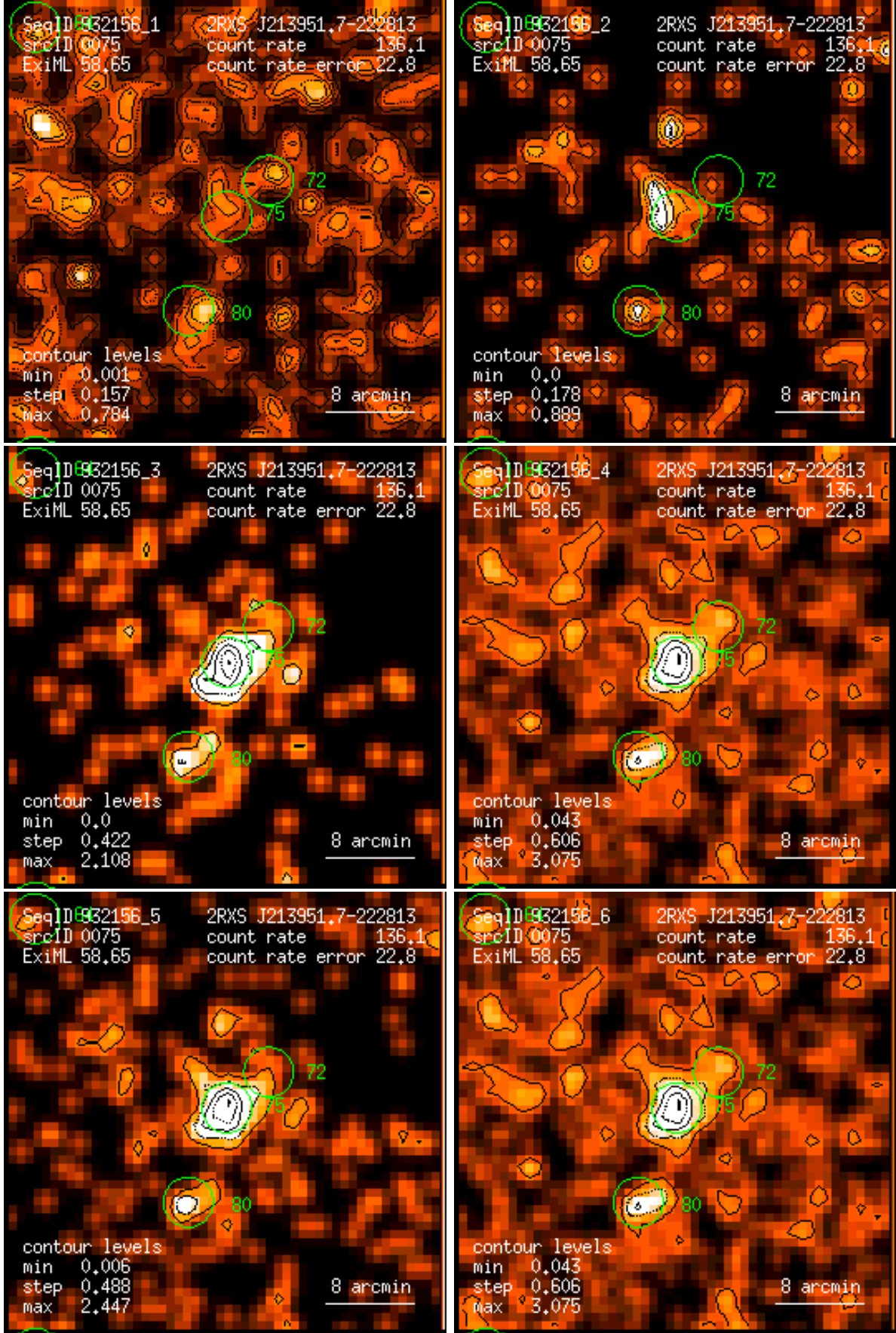
Figure 75: RASS 932156: detection 0075: band rate images, Gaussian filter: (1) PSPC channels 11 – 41, (2) 52 – 90, (3) 91 – 201, (4) 11 – 235, (5) 52 – 201, (6) 11 – 201. Broad band rates in counts/ks. Band rate contour levels in counts/ks/arcmin 2 .
