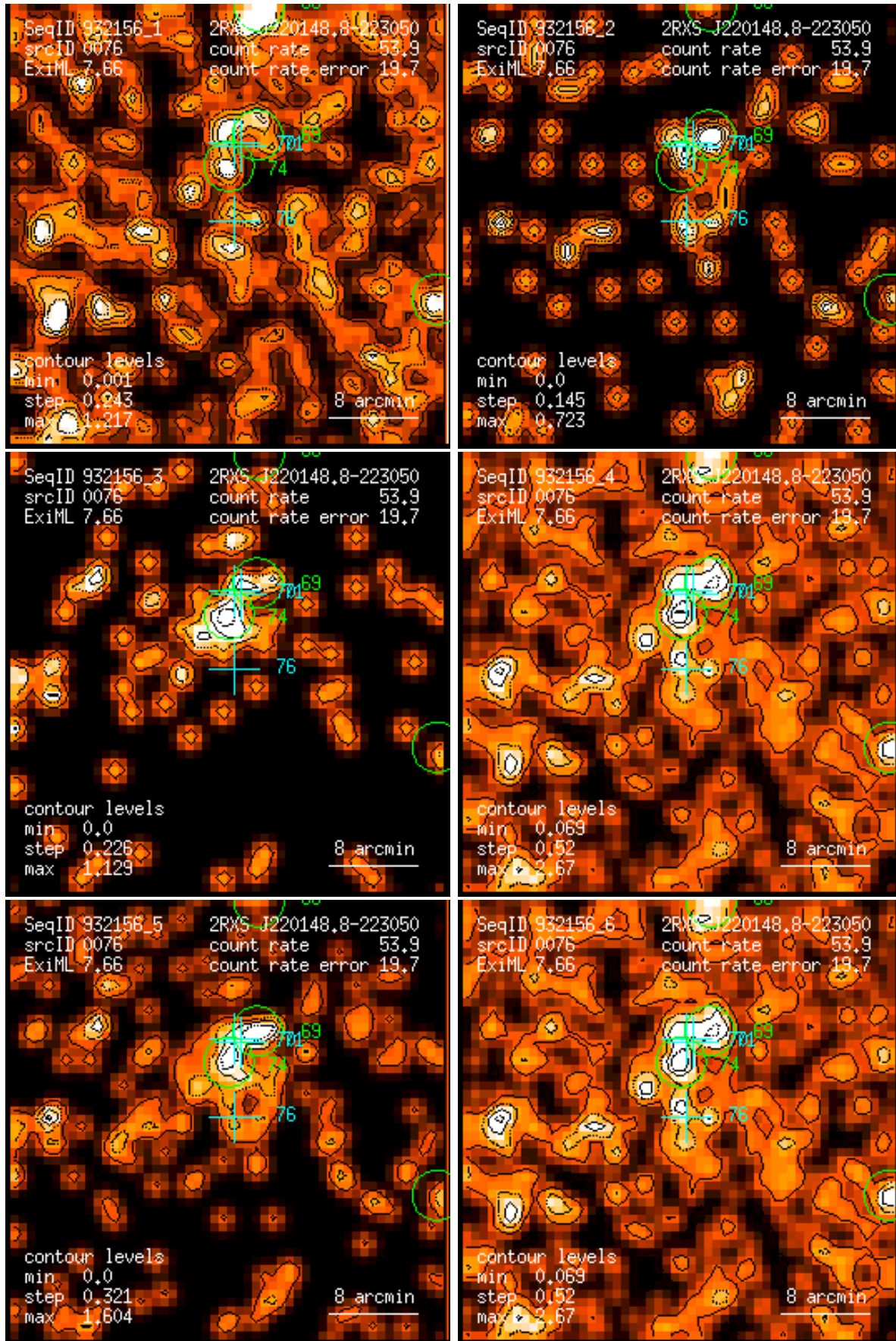
Figure 76: RASS 932156: detection 0076: band rate images, Gaussian filter: (1) PSPC channels 11 – 41, (2) 52 – 90, (3) 91 – 201, (4) 11 – 235, (5) 52 – 201, (6) 11 – 201. Broad band rates in counts/ks. Band rate contour levels in counts/ks/arcmin 2 .
