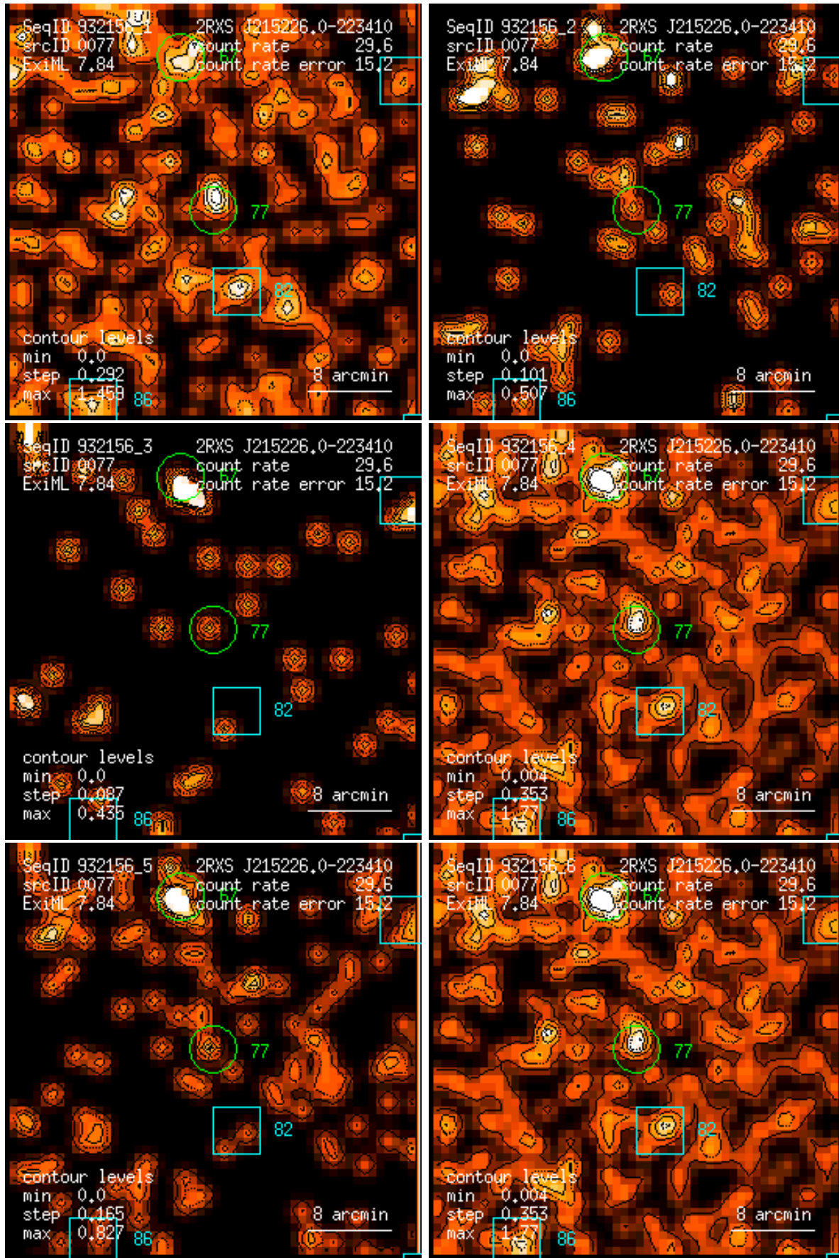
Figure 77: RASS 932156: detection 0077: band rate images, Gaussian filter: (1) PSPC channels 11 – 41, (2) 52 – 90, (3) 91 – 201, (4) 11 – 235, (5) 52 – 201, (6) 11 – 201. Broad band rates in counts/ks. Band rate contour levels in counts/ks/arcmin 2 .
