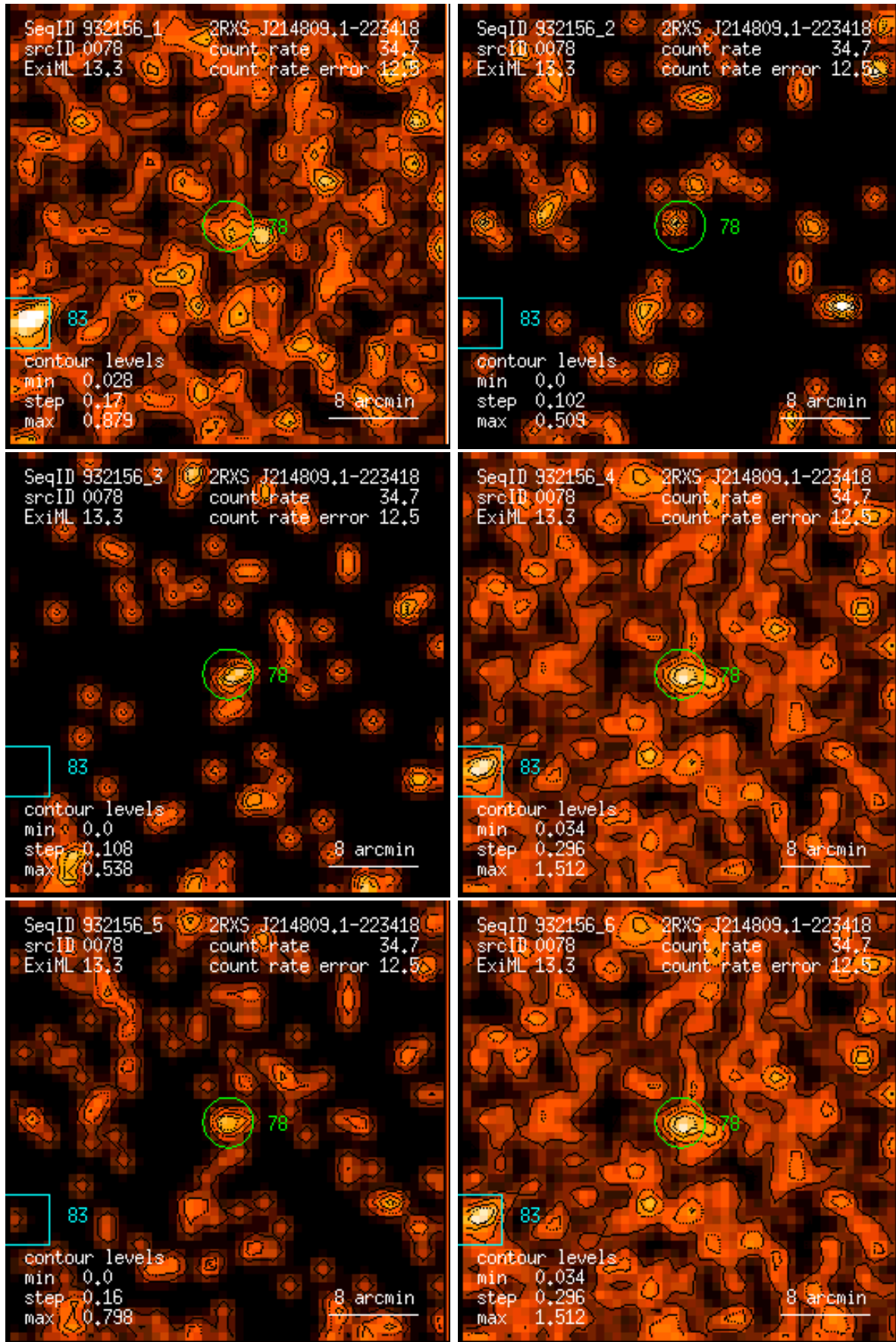
Figure 78: RASS 932156: detection 0078: band rate images, Gaussian filter: (1) PSPC channels 11 – 41, (2) 52 – 90, (3) 91 – 201, (4) 11 – 235, (5) 52 – 201, (6) 11 – 201. Broad band rates in counts/ks. Band rate contour levels in counts/ks/arcmin 2 .
