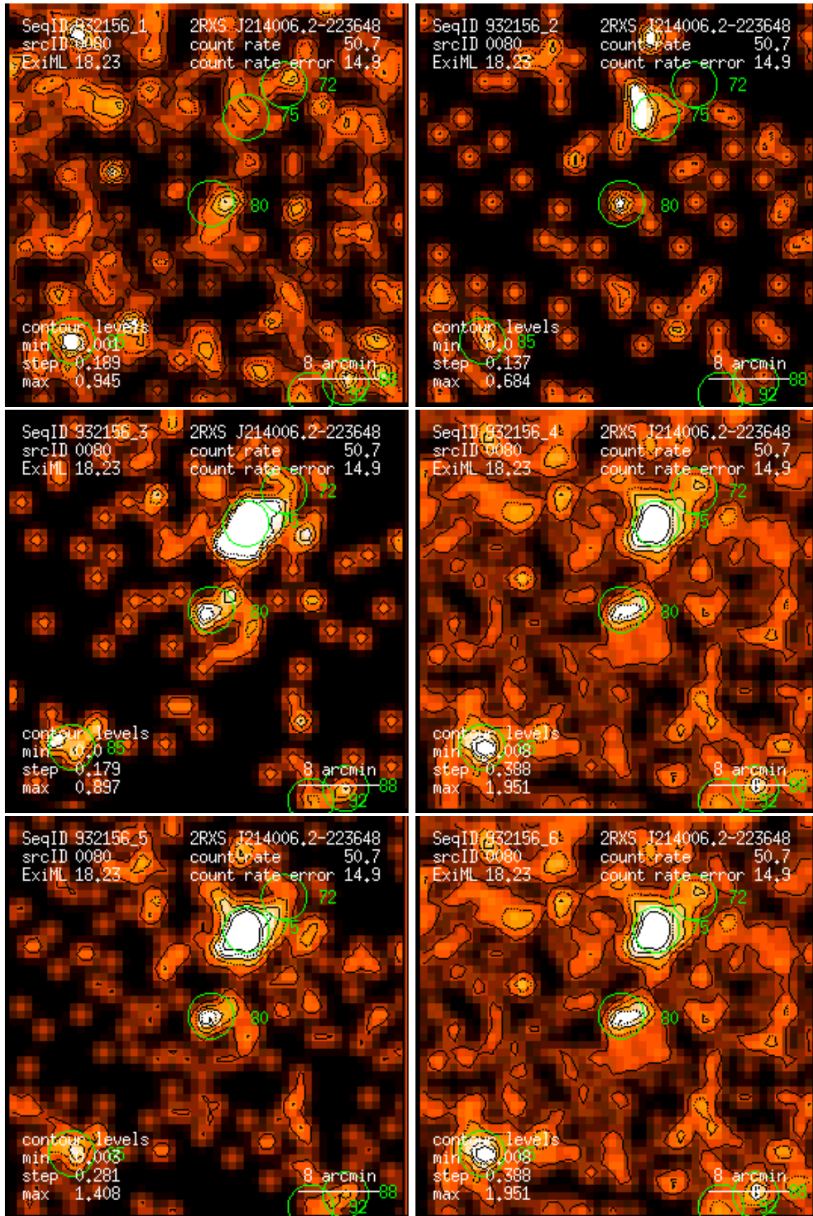
Figure 80: RASS 932156: detection 0080: band rate images, Gaussian filter: (1) PSPC channels 11 – 41, (2) 52 – 90, (3) 91 – 201, (4) 11 – 235, (5) 52 – 201, (6) 11 – 201. Broad band rates in counts/ks. Band rate contour levels in counts/ks/arcmin 2 .
