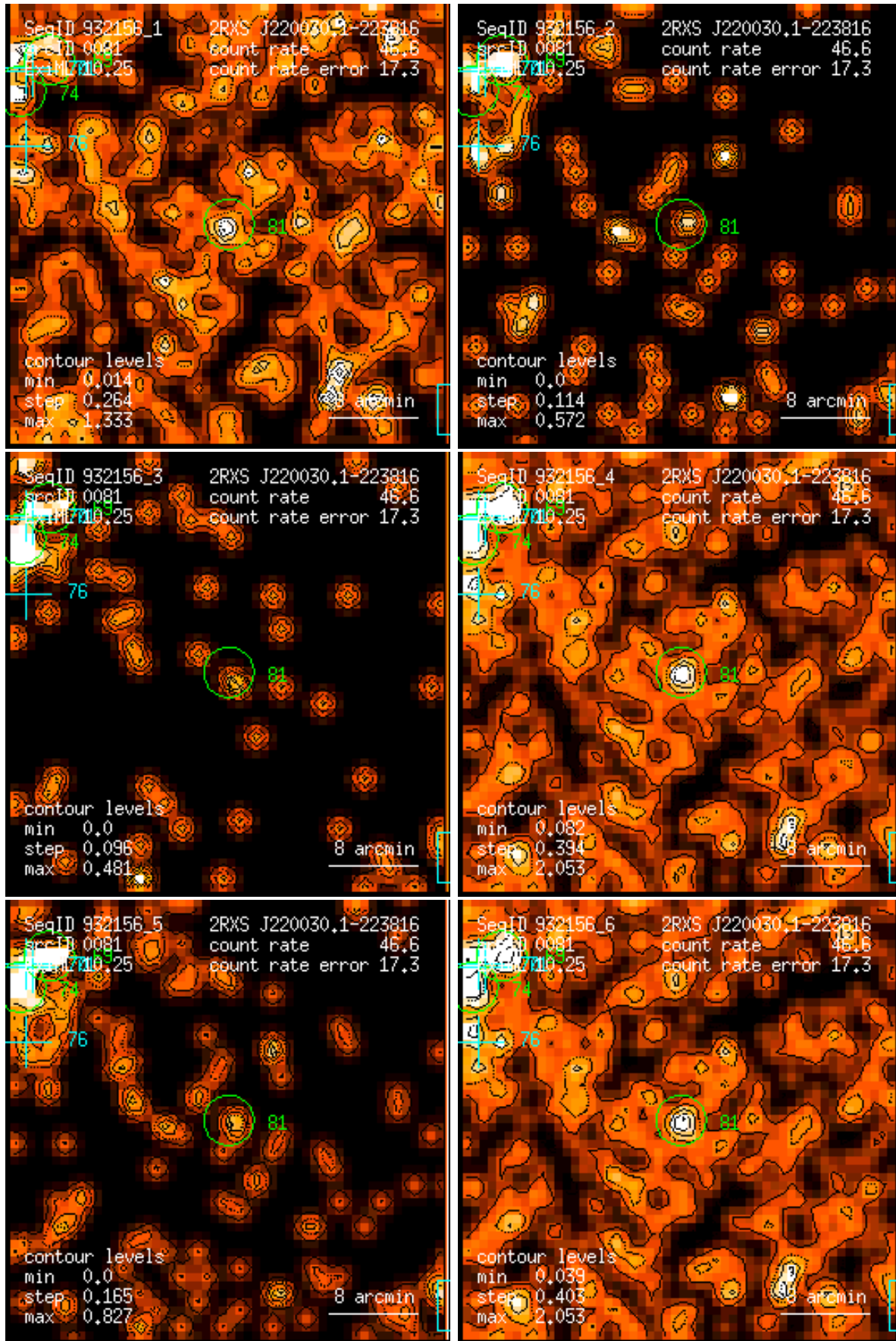
Figure 81: RASS 932156: detection 0081: band rate images, Gaussian filter: (1) PSPC channels 11 – 41, (2) 52 – 90, (3) 91 – 201, (4) 11 – 235, (5) 52 – 201, (6) 11 – 201. Broad band rates in counts/ks. Band rate contour levels in counts/ks/arcmin 2 .
