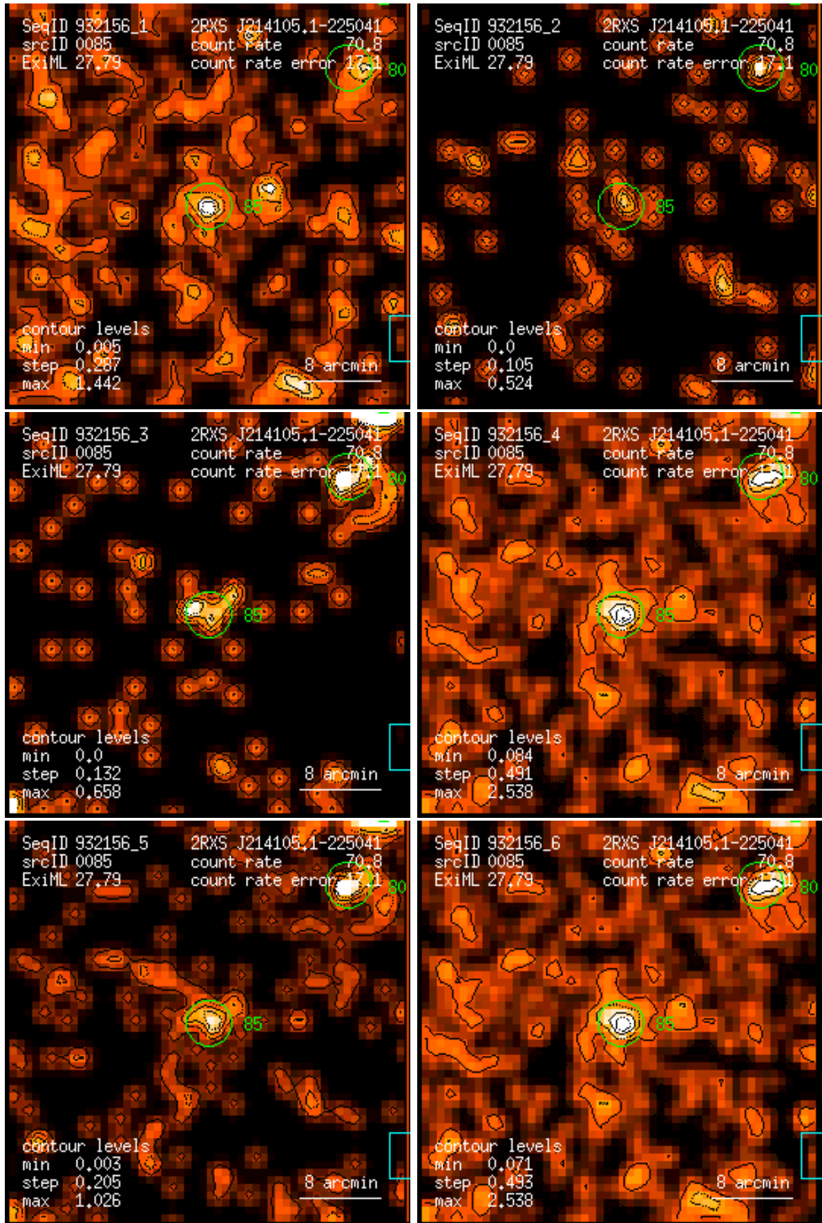
Figure 85: RASS 932156: detection 0085: band rate images, Gaussian filter: (1) PSPC channels 11 – 41, (2) 52 – 90, (3) 91 – 201, (4) 11 – 235, (5) 52 – 201, (6) 11 – 201. Broad band rates in counts/ks. Band rate contour levels in counts/ks/arcmin 2 .
