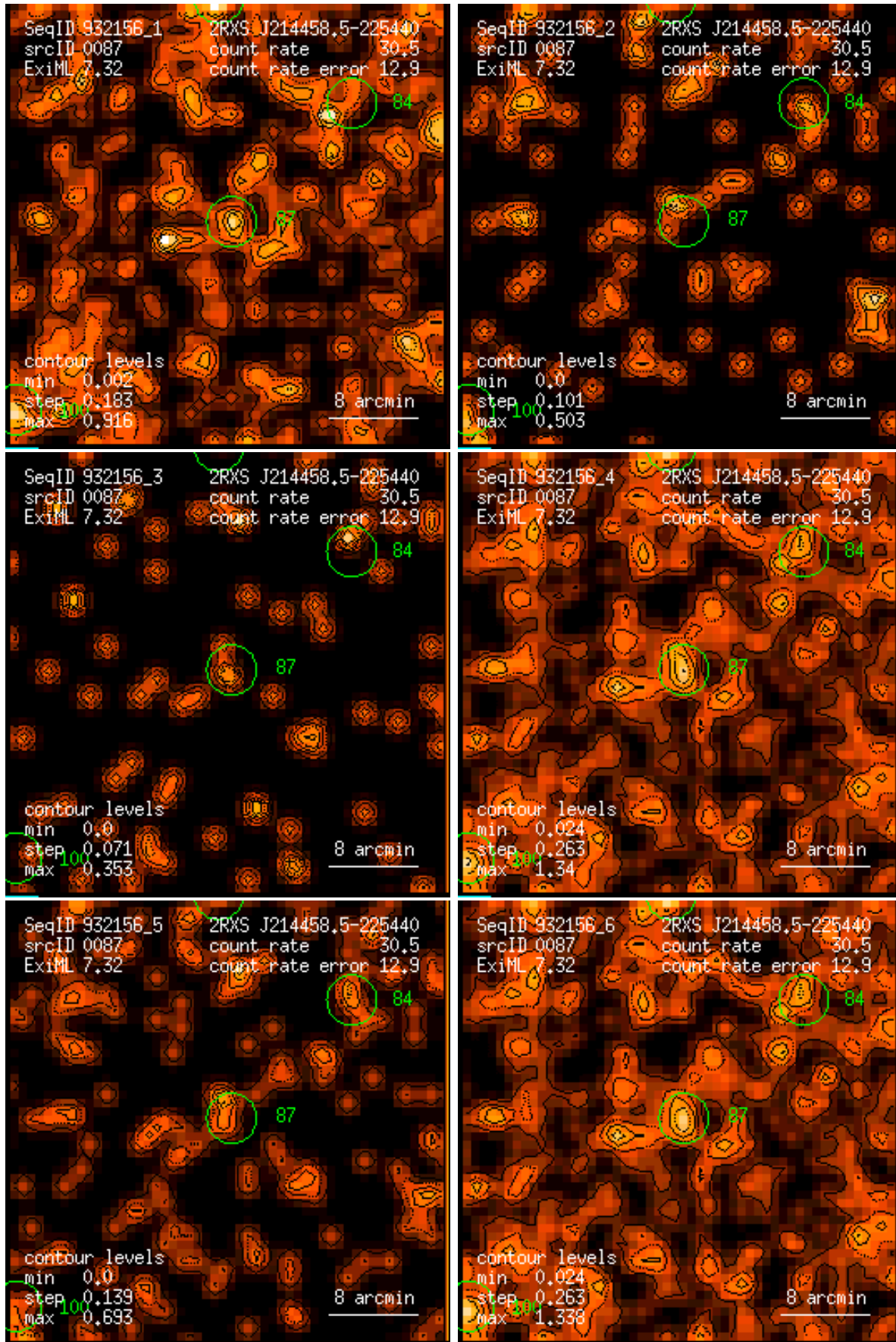
Figure 87: RASS 932156: detection 0087: band rate images, Gaussian filter: (1) PSPC channels 11 – 41, (2) 52 – 90, (3) 91 – 201, (4) 11 – 235, (5) 52 – 201, (6) 11 – 201. Broad band rates in counts/ks. Band rate contour levels in counts/ks/arcmin 2 .
