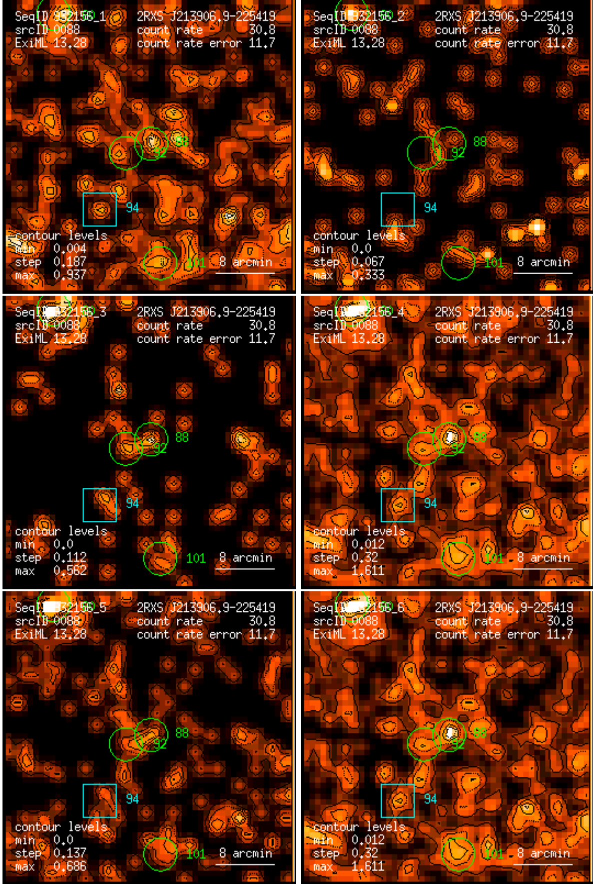
Figure 88: RASS 932156: detection 0088: band rate images, Gaussian filter: (1) PSPC channels 11 – 41, (2) 52 – 90, (3) 91 – 201, (4) 11 – 235, (5) 52 – 201, (6) 11 – 201. Broad band rates in counts/ks. Band rate contour levels in counts/ks/arcmin 2 .
