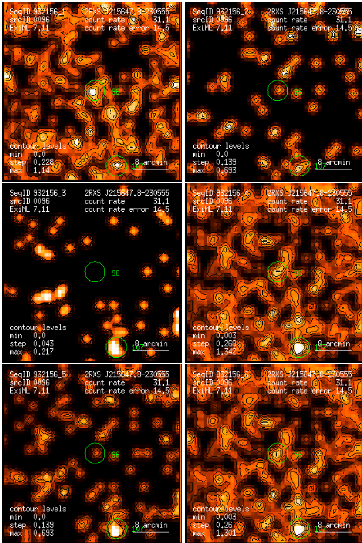
Figure 96: RASS 932156: detection 0096: band rate images, Gaussian filter: (1) PSPC channels 11 – 41, (2) 52 – 90, (3) 91 – 201, (4) 11 – 235, (5) 52 – 201, (6) 11 – 201. Broad band rates in counts/ks. Band rate contour levels in counts/ks/arcmin 2 .
