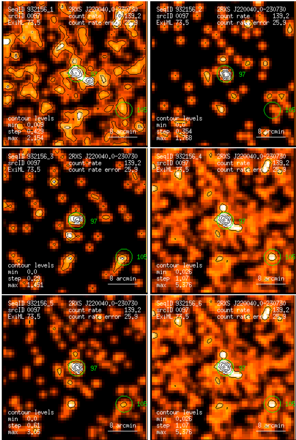
Figure 97: RASS 932156: detection 0097: band rate images, Gaussian filter: (1) PSPC channels 11 – 41, (2) 52 – 90, (3) 91 – 201, (4) 11 – 235, (5) 52 – 201, (6) 11 – 201. Broad band rates in counts/ks. Band rate contour levels in counts/ks/arcmin 2 .
