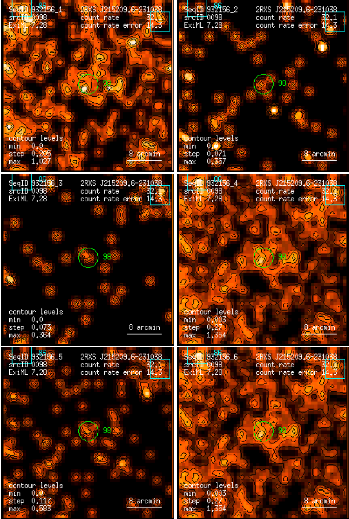
Figure 98: RASS 932156: detection 0098: band rate images, Gaussian filter: (1) PSPC channels 11 – 41, (2) 52 – 90, (3) 91 – 201, (4) 11 – 235, (5) 52 – 201, (6) 11 – 201. Broad band rates in counts/ks. Band rate contour levels in counts/ks/arcmin 2 .
