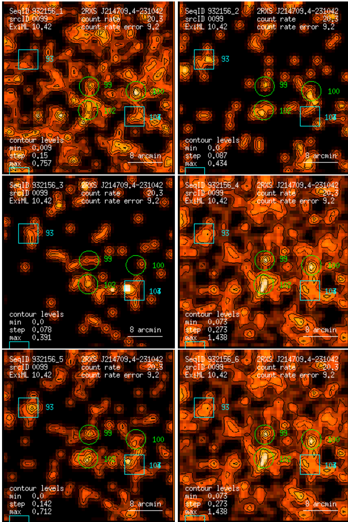
Figure 99: RASS 932156: detection 0099: band rate images, Gaussian filter: (1) PSPC channels 11 – 41, (2) 52 – 90, (3) 91 – 201, (4) 11 – 235, (5) 52 – 201, (6) 11 – 201. Broad band rates in counts/ks. Band rate contour levels in counts/ks/arcmin 2 .
