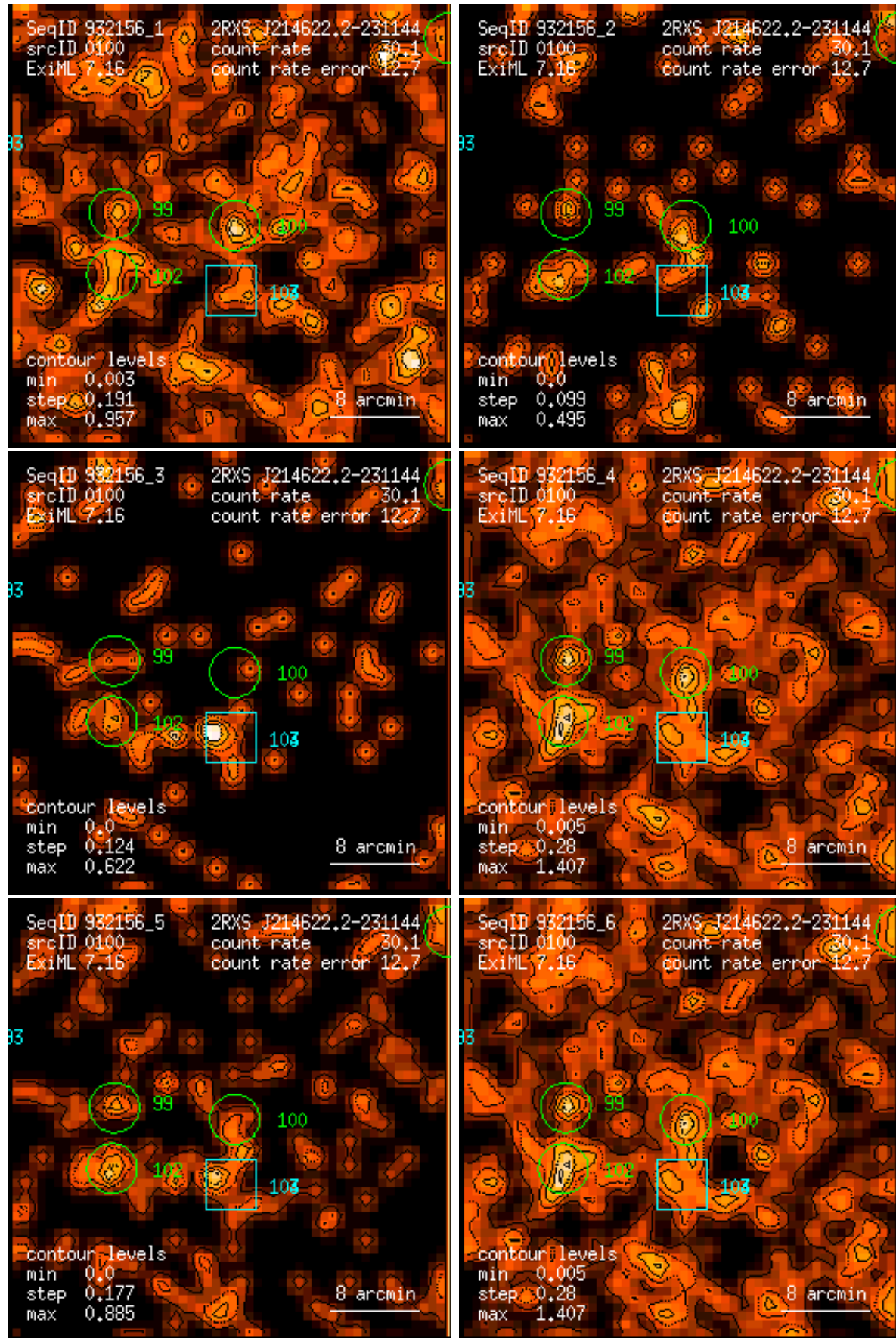
Figure 100: RASS 932156: detection 0100: band rate images, Gaussian filter: (1) PSPC channels 11 – 41, (2) 52 – 90, (3) 91 – 201, (4) 11 – 235, (5) 52 – 201, (6) 11 – 201. Broad band rates in counts/ks. Band rate contour levels in counts/ks/arcmin 2 .
