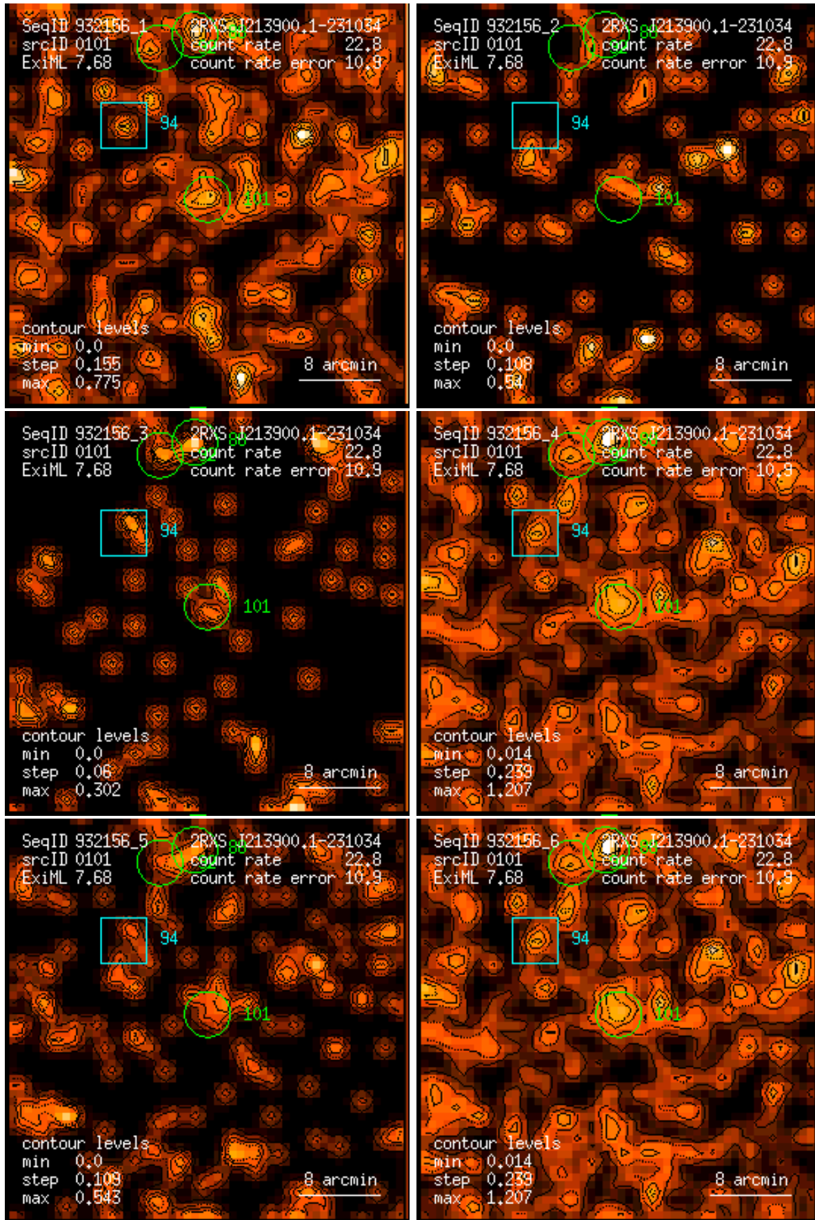
Figure 101: RASS 932156: detection 0101: band rate images, Gaussian filter: (1) PSPC channels 11 – 41, (2) 52 – 90, (3) 91 – 201, (4) 11 – 235, (5) 52 – 201, (6) 11 – 201. Broad band rates in counts/ks. Band rate contour levels in counts/ks/arcmin 2 .
