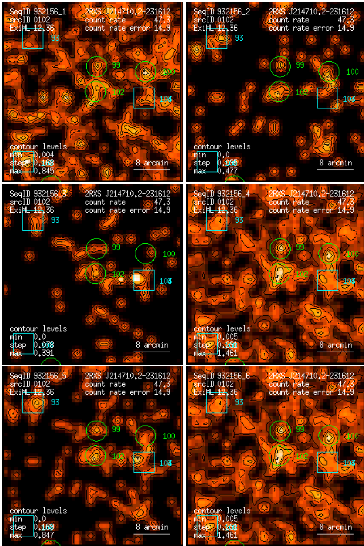
Figure 102: RASS 932156: detection 0102: band rate images, Gaussian filter: (1) PSPC channels 11 – 41, (2) 52 – 90, (3) 91 – 201, (4) 11 – 235, (5) 52 – 201, (6) 11 – 201. Broad band rates in counts/ks. Band rate contour levels in counts/ks/arcmin 2 .
