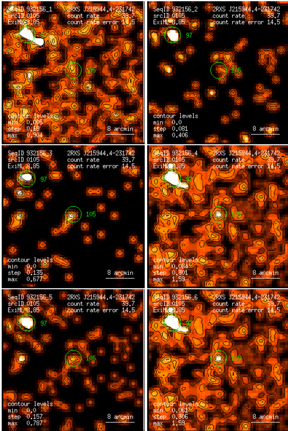
Figure 105: RASS 932156: detection 0105: band rate images, Gaussian filter: (1) PSPC channels 11 – 41, (2) 52 – 90, (3) 91 – 201, (4) 11 – 235, (5) 52 – 201, (6) 11 – 201. Broad band rates in counts/ks. Band rate contour levels in counts/ks/arcmin 2 .
