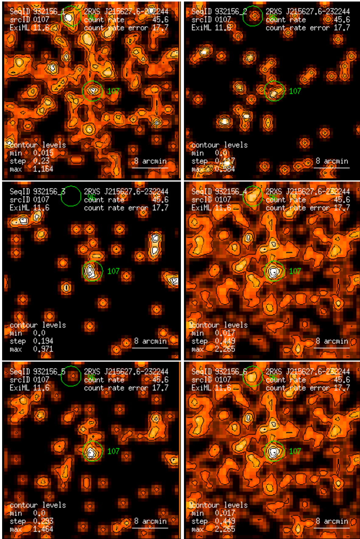
Figure 107: RASS 932156: detection 0107: band rate images, Gaussian filter: (1) PSPC channels 11 – 41, (2) 52 – 90, (3) 91 – 201, (4) 11 – 235, (5) 52 – 201, (6) 11 – 201. Broad band rates in counts/ks. Band rate contour levels in counts/ks/arcmin 2 .
