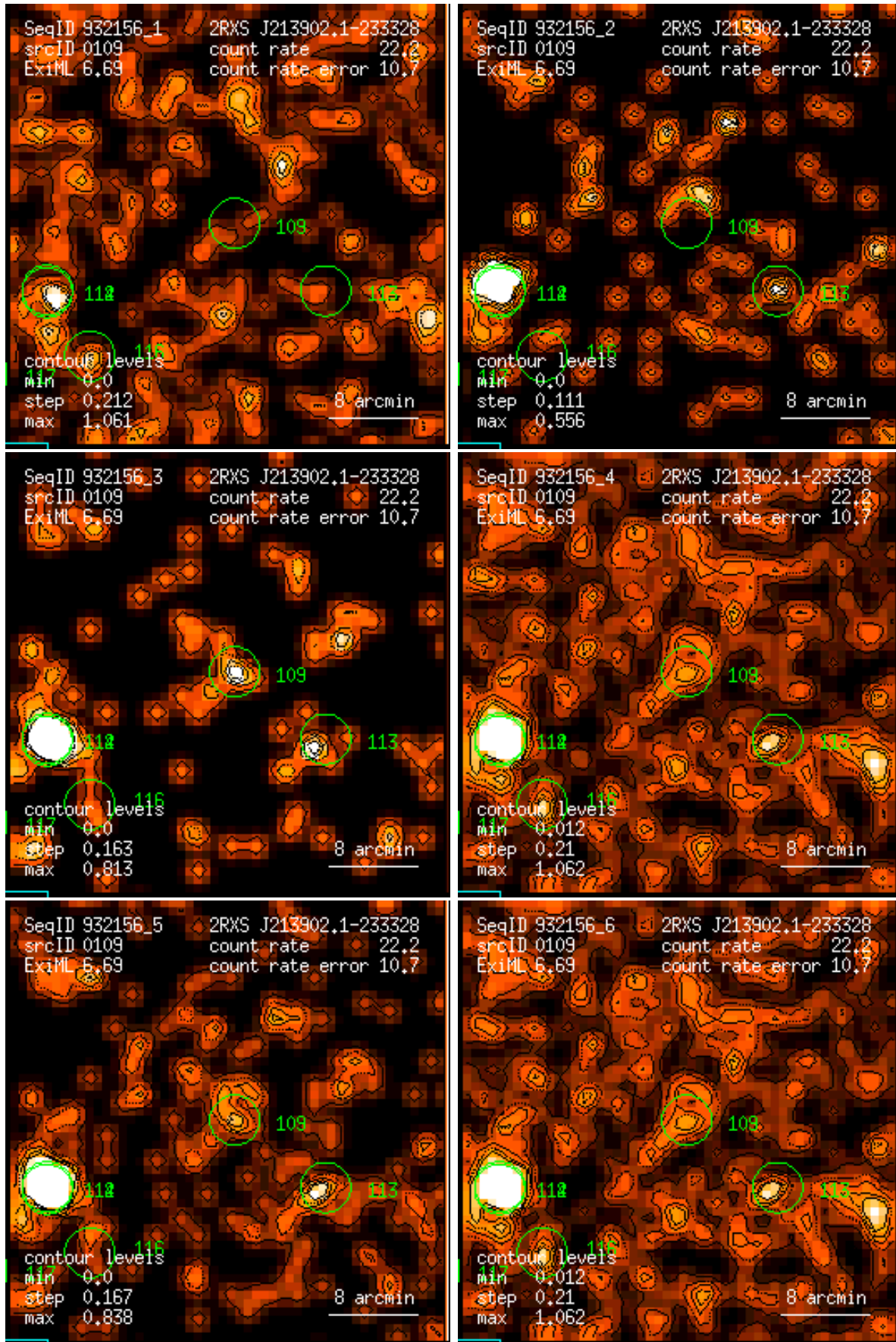
Figure 109: RASS 932156: detection 0109: band rate images, Gaussian filter: (1) PSPC channels 11 – 41, (2) 52 – 90, (3) 91 – 201, (4) 11 – 235, (5) 52 – 201, (6) 11 – 201. Broad band rates in counts/ks. Band rate contour levels in counts/ks/arcmin 2 .
