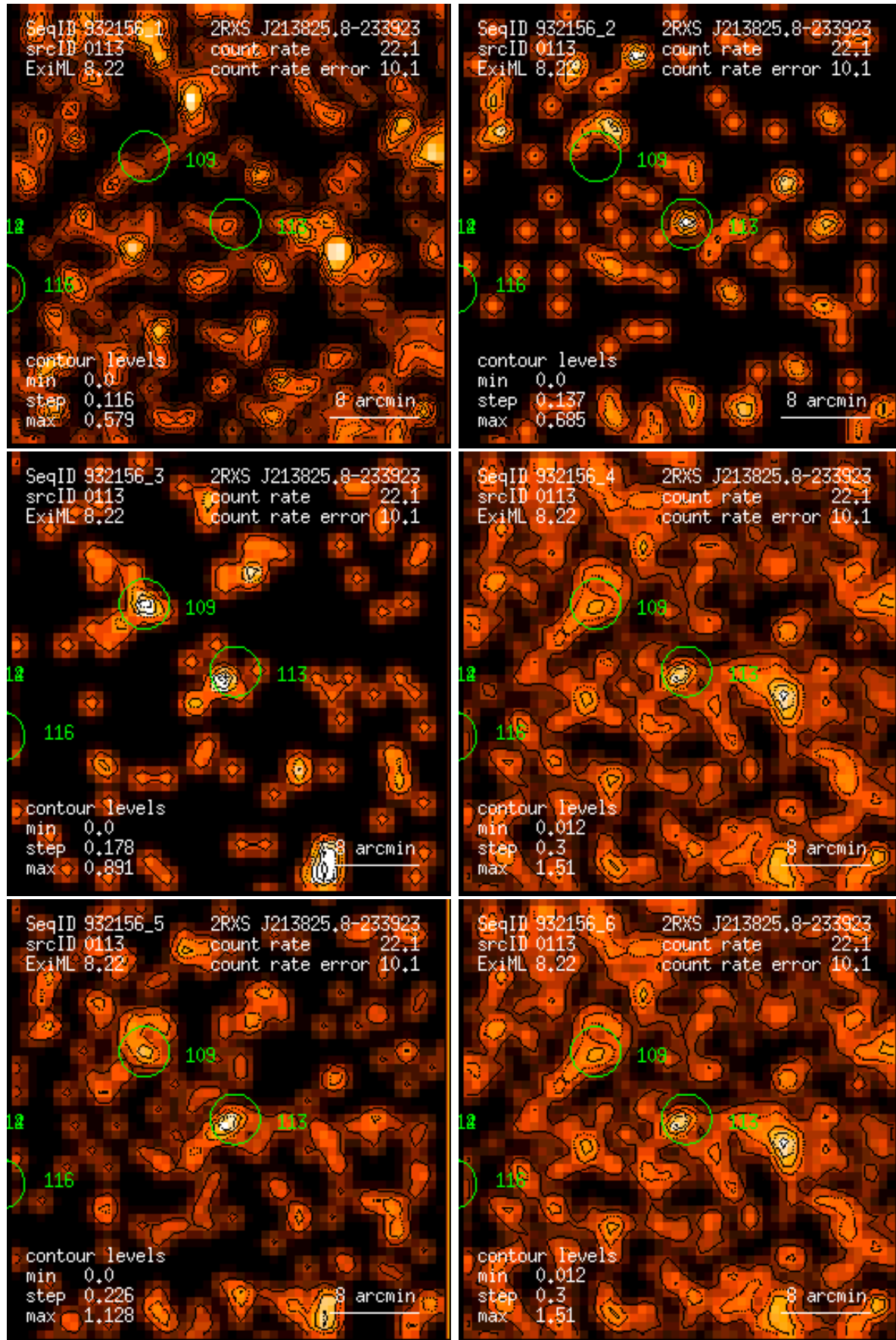
Figure 113: RASS 932156: detection 0113: band rate images, Gaussian filter: (1) PSPC channels 11 – 41, (2) 52 – 90, (3) 91 – 201, (4) 11 – 235, (5) 52 – 201, (6) 11 – 201. Broad band rates in counts/ks. Band rate contour levels in counts/ks/arcmin 2 .
