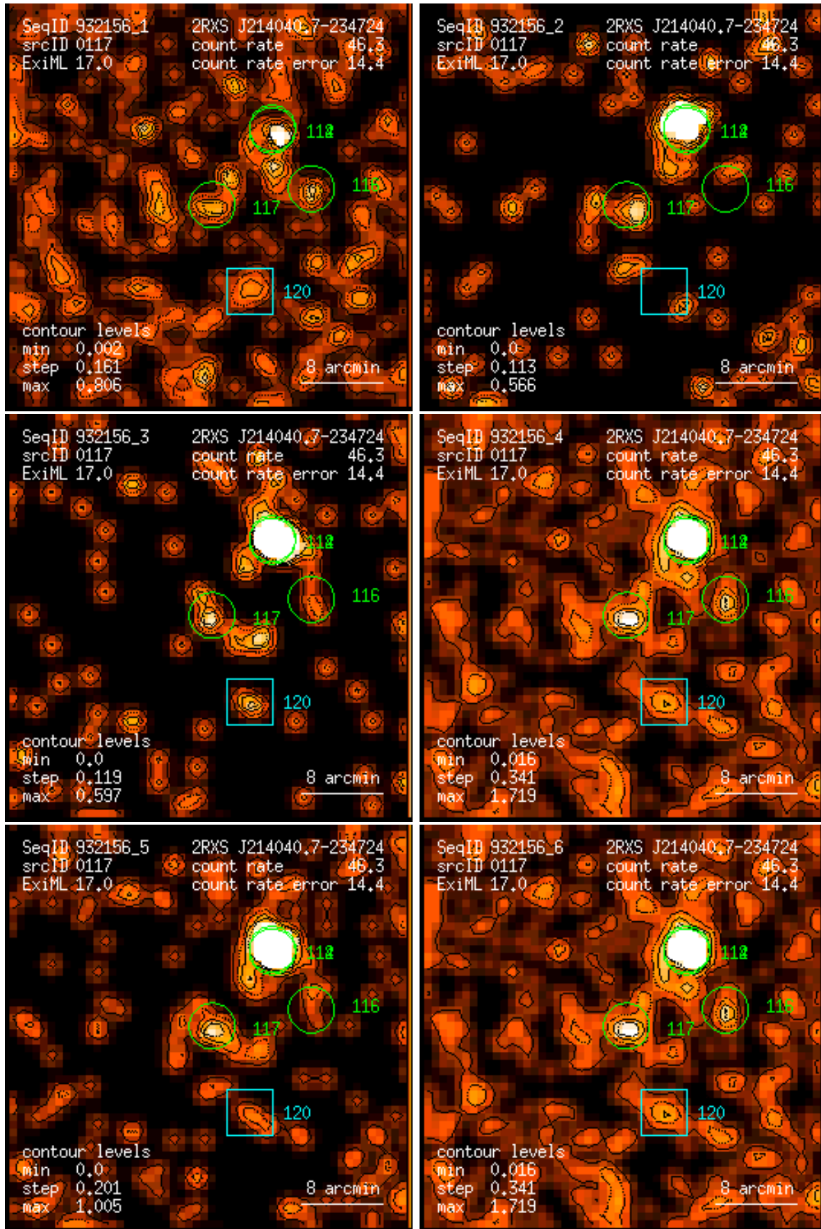
Figure 117: RASS 932156: detection 0117: band rate images, Gaussian filter: (1) PSPC channels 11 – 41, (2) 52 – 90, (3) 91 – 201, (4) 11 – 235, (5) 52 – 201, (6) 11 – 201. Broad band rates in counts/ks. Band rate contour levels in counts/ks/arcmin 2 .
