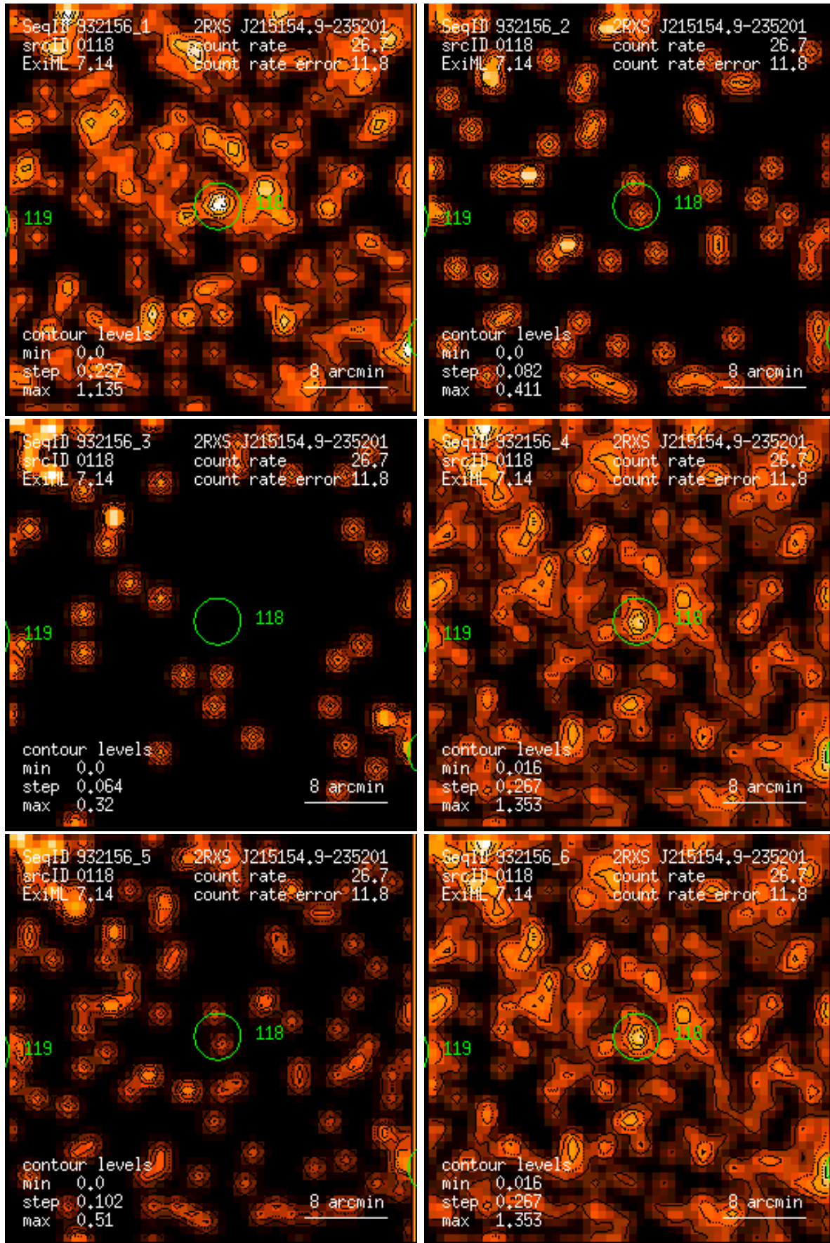
Figure 118: RASS 932156: detection 0118: band rate images, Gaussian filter: (1) PSPC channels 11 – 41, (2) 52 – 90, (3) 91 – 201, (4) 11 – 235, (5) 52 – 201, (6) 11 – 201. Broad band rates in counts/ks. Band rate contour levels in counts/ks/arcmin 2 .
