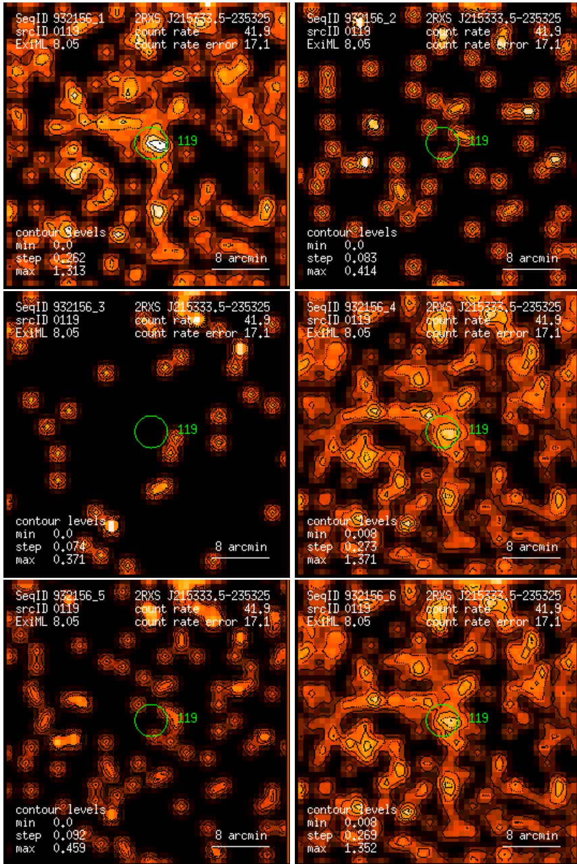
Figure 119: RASS 932156: detection 0119: band rate images, Gaussian filter: (1) PSPC channels 11 – 41, (2) 52 – 90, (3) 91 – 201, (4) 11 – 235, (5) 52 – 201, (6) 11 – 201. Broad band rates in counts/ks. Band rate contour levels in counts/ks/arcmin 2 .
