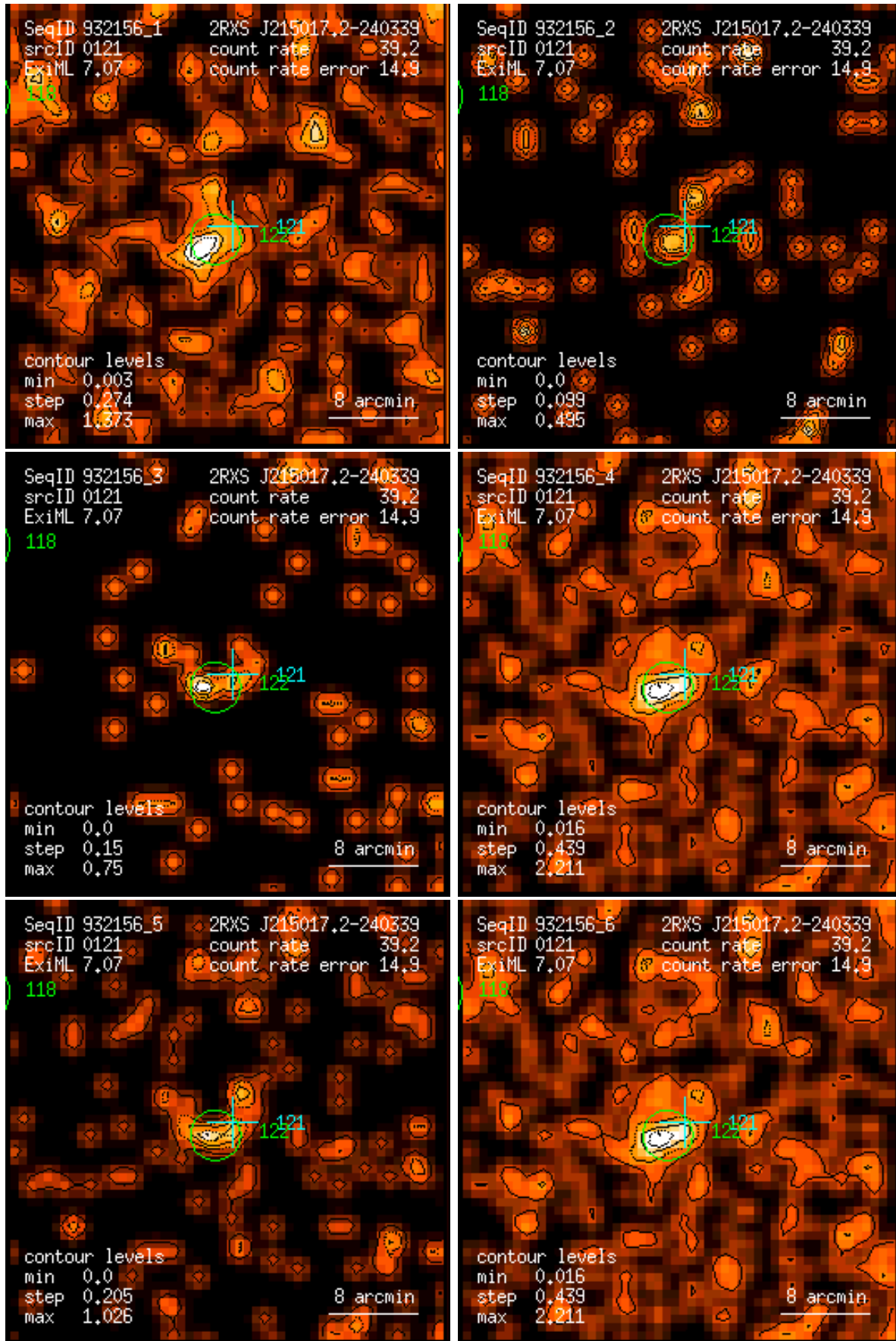
Figure 121: RASS 932156: detection 0121: band rate images, Gaussian filter: (1) PSPC channels 11 – 41, (2) 52 – 90, (3) 91 – 201, (4) 11 – 235, (5) 52 – 201, (6) 11 – 201. Broad band rates in counts/ks. Band rate contour levels in counts/ks/arcmin 2 .
