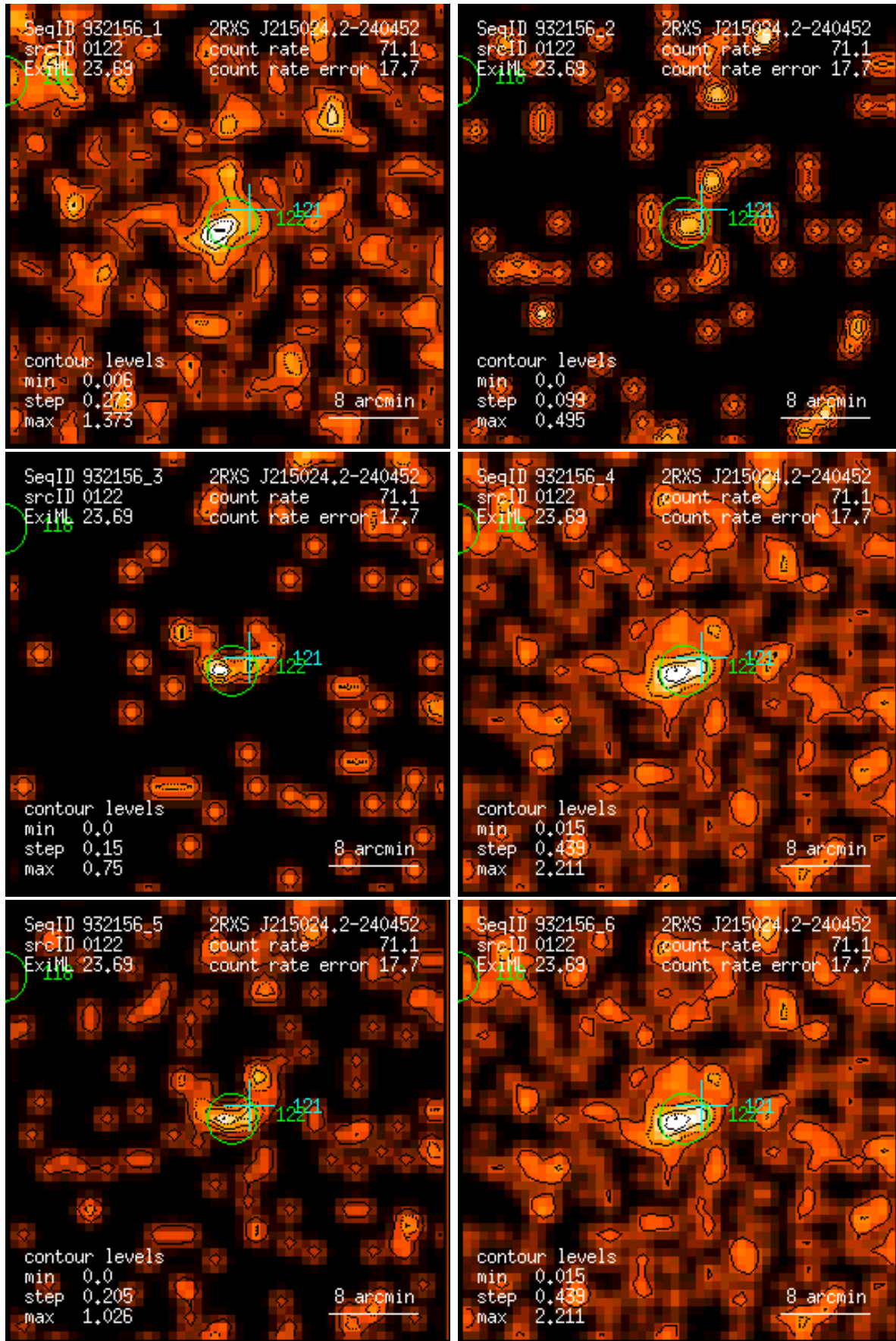
Figure 122: RASS 932156: detection 0122: band rate images, Gaussian filter: (1) PSPC channels 11 – 41, (2) 52 – 90, (3) 91 – 201, (4) 11 – 235, (5) 52 – 201, (6) 11 – 201. Broad band rates in counts/ks. Band rate contour levels in counts/ks/arcmin 2 .
