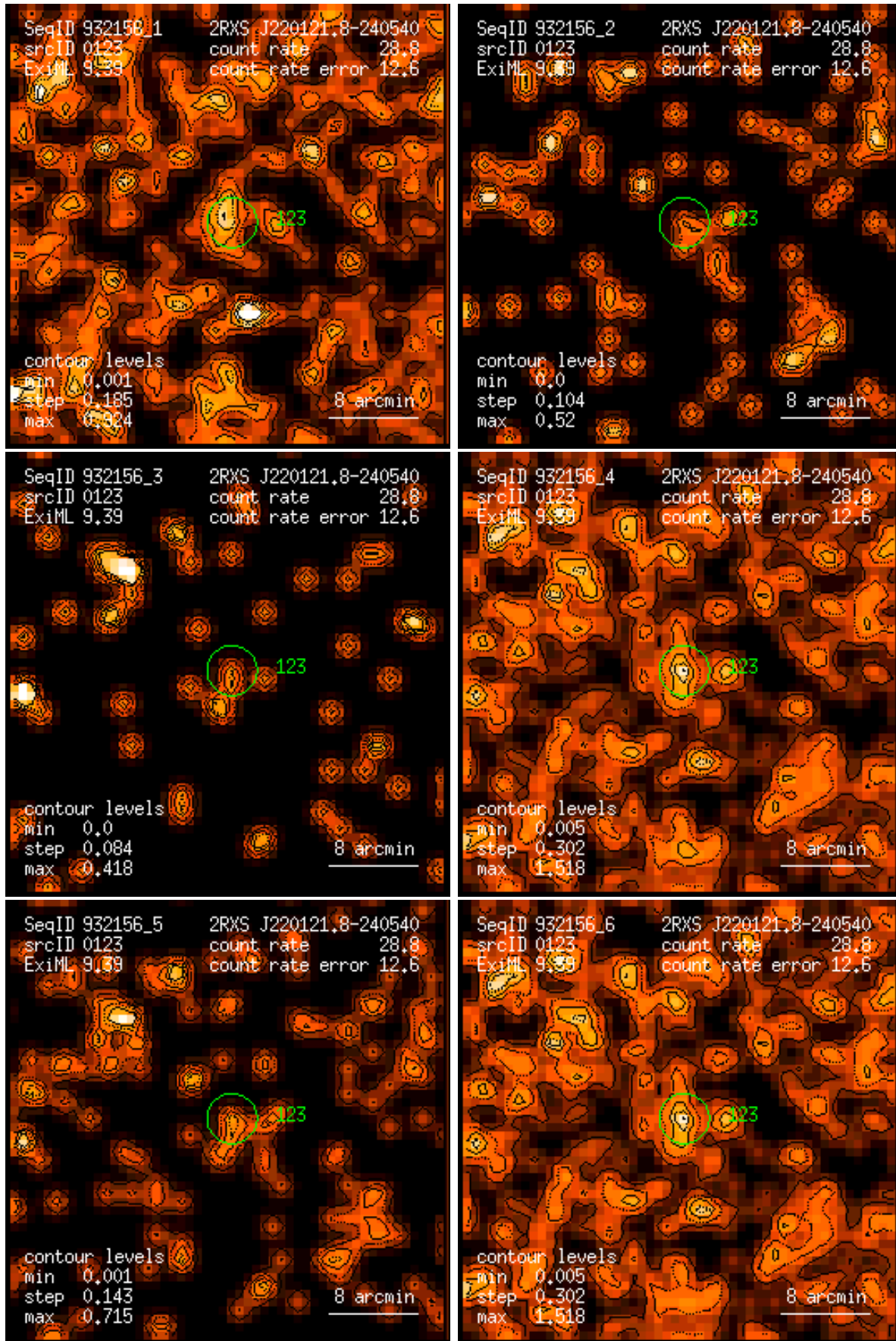
Figure 123: RASS 932156: detection 0123: band rate images, Gaussian filter: (1) PSPC channels 11 – 41, (2) 52 – 90, (3) 91 – 201, (4) 11 – 235, (5) 52 – 201, (6) 11 – 201. Broad band rates in counts/ks. Band rate contour levels in counts/ks/arcmin 2 .
