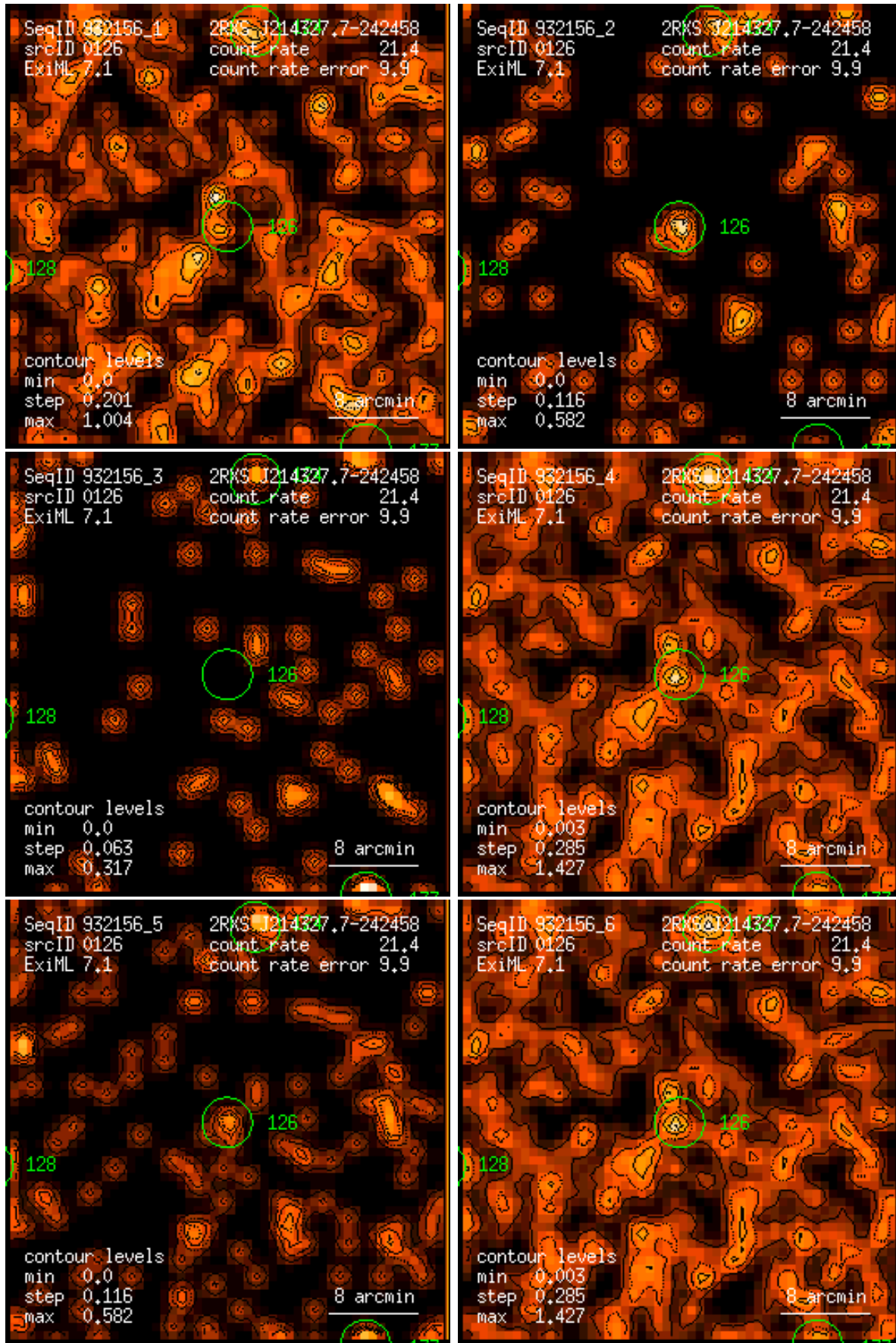
Figure 126: RASS 932156: detection 0126: band rate images, Gaussian filter: (1) PSPC channels 11 – 41, (2) 52 – 90, (3) 91 – 201, (4) 11 – 235, (5) 52 – 201, (6) 11 – 201. Broad band rates in counts/ks. Band rate contour levels in counts/ks/arcmin 2 .
