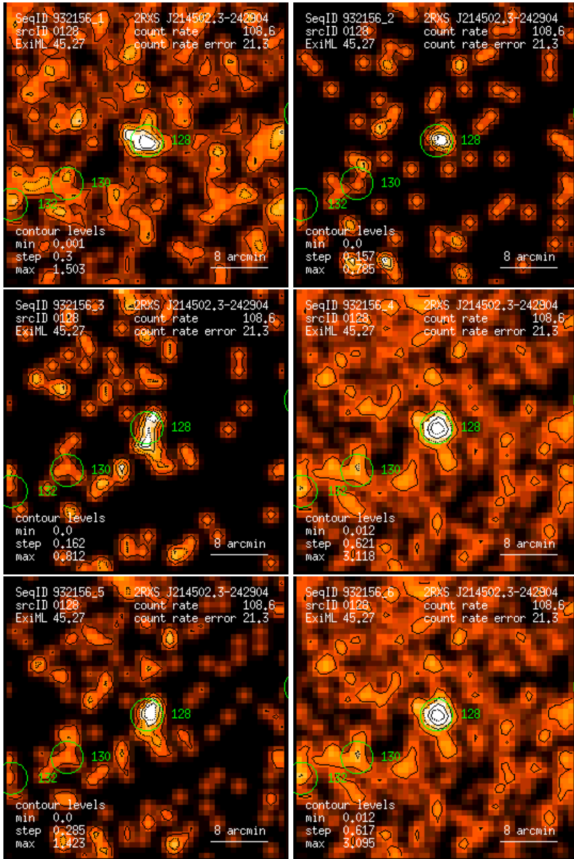
Figure 128: RASS 932156: detection 0128: band rate images, Gaussian filter: (1) PSPC channels 11 – 41, (2) 52 – 90, (3) 91 – 201, (4) 11 – 235, (5) 52 – 201, (6) 11 – 201. Broad band rates in counts/ks. Band rate contour levels in counts/ks/arcmin 2 .
