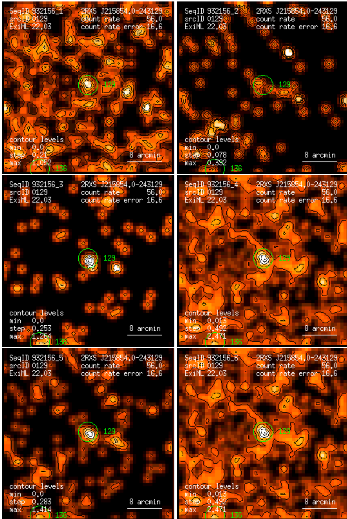
Figure 129: RASS 932156: detection 0129: band rate images, Gaussian filter: (1) PSPC channels 11 – 41, (2) 52 – 90, (3) 91 – 201, (4) 11 – 235, (5) 52 – 201, (6) 11 – 201. Broad band rates in counts/ks. Band rate contour levels in counts/ks/arcmin 2 .
