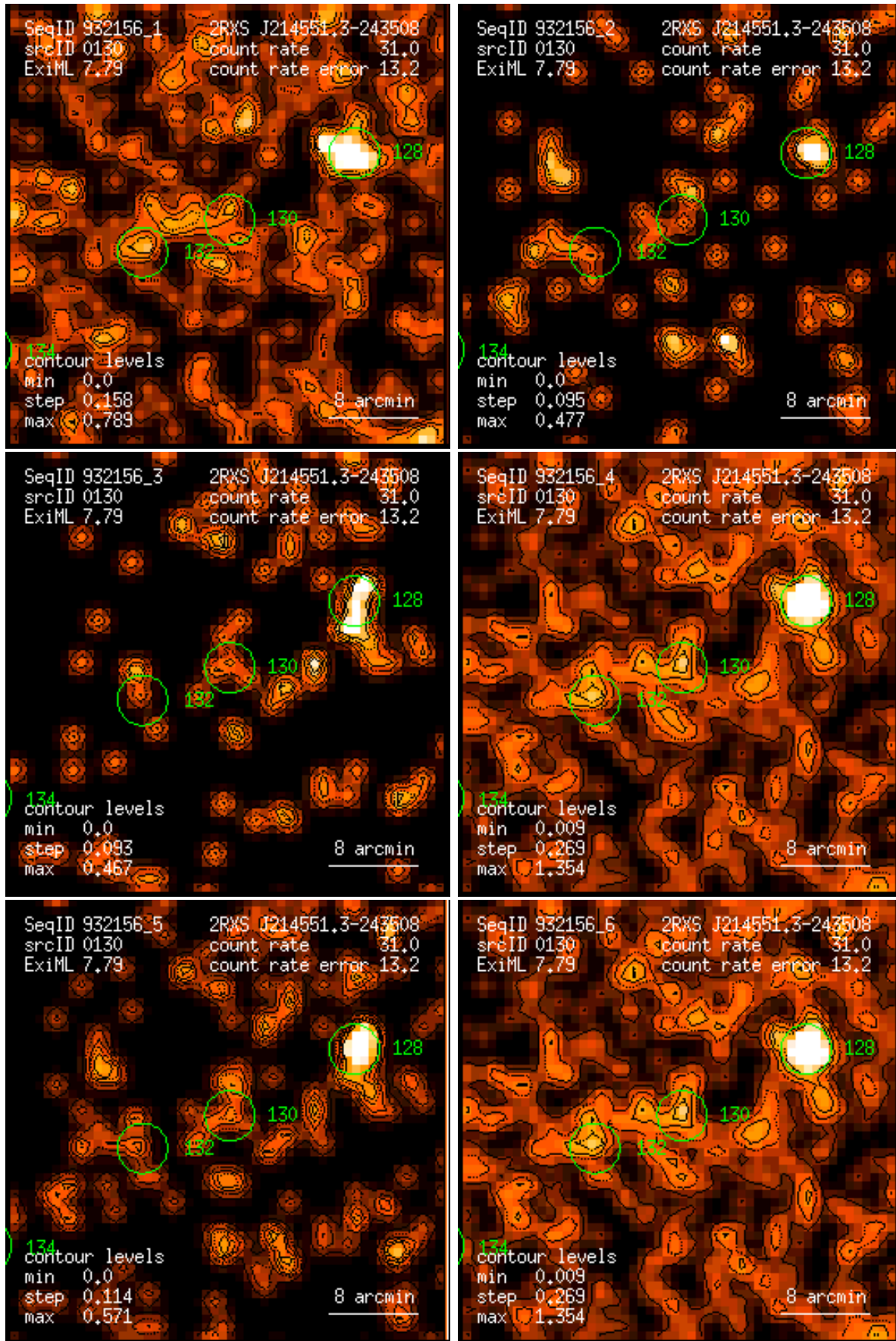
Figure 130: RASS 932156: detection 0130: band rate images, Gaussian filter: (1) PSPC channels 11 – 41, (2) 52 – 90, (3) 91 – 201, (4) 11 – 235, (5) 52 – 201, (6) 11 – 201. Broad band rates in counts/ks. Band rate contour levels in counts/ks/arcmin 2 .
