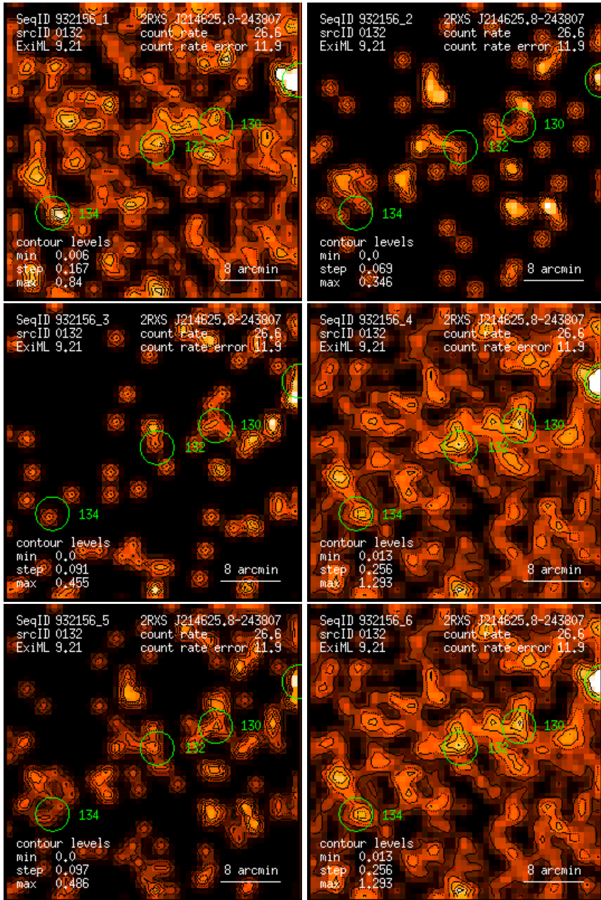
Figure 132: RASS 932156: detection 0132: band rate images, Gaussian filter: (1) PSPC channels 11 – 41, (2) 52 – 90, (3) 91 – 201, (4) 11 – 235, (5) 52 – 201, (6) 11 – 201. Broad band rates in counts/ks. Band rate contour levels in counts/ks/arcmin 2 .
