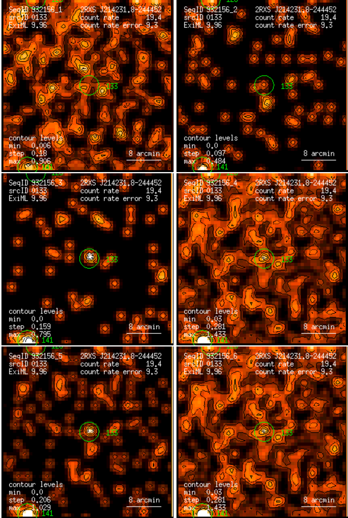
Figure 133: RASS 932156: detection 0133: band rate images, Gaussian filter: (1) PSPC channels 11 – 41, (2) 52 – 90, (3) 91 – 201, (4) 11 – 235, (5) 52 – 201, (6) 11 – 201. Broad band rates in counts/ks. Band rate contour levels in counts/ks/arcmin 2 .
